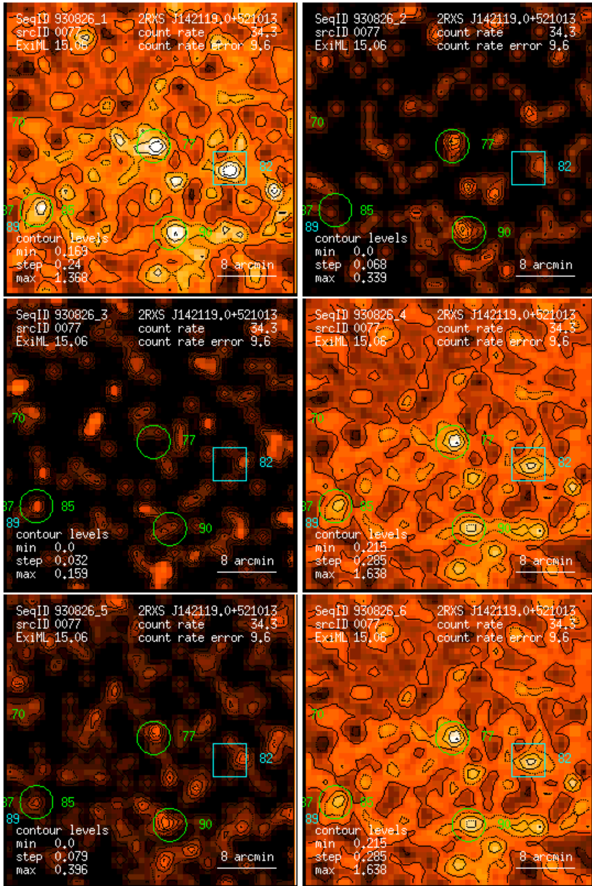
Figure 77: RASS 930826: detection 0077: band rate images, Gaussian filter: (1) PSPC channels 11 – 41, (2) 52 – 90, (3) 91 – 201, (4) 11 – 235, (5) 52 – 201, (6) 11 – 201. Broad band rates in counts/ks. Band rate contour levels in counts/ks/arcmin 2 .
