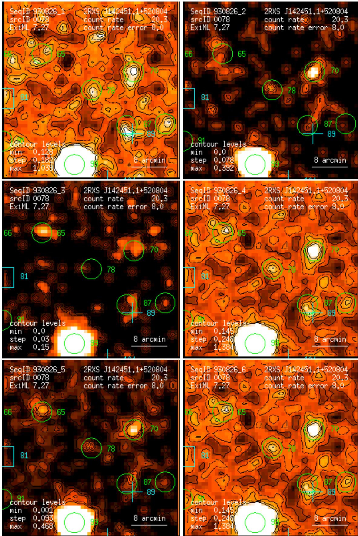
Figure 78: RASS 930826: detection 0078: band rate images, Gaussian filter: (1) PSPC channels 11 – 41, (2) 52 – 90, (3) 91 – 201, (4) 11 – 235, (5) 52 – 201, (6) 11 – 201. Broad band rates in counts/ks. Band rate contour levels in counts/ks/arcmin 2 .
