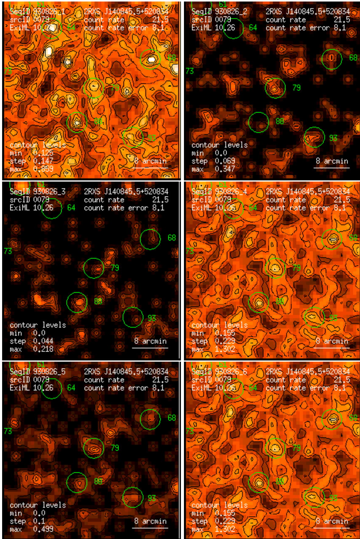
Figure 79: RASS 930826: detection 0079: band rate images, Gaussian filter: (1) PSPC channels 11 – 41, (2) 52 – 90, (3) 91 – 201, (4) 11 – 235, (5) 52 – 201, (6) 11 – 201. Broad band rates in counts/ks. Band rate contour levels in counts/ks/arcmin 2 .
