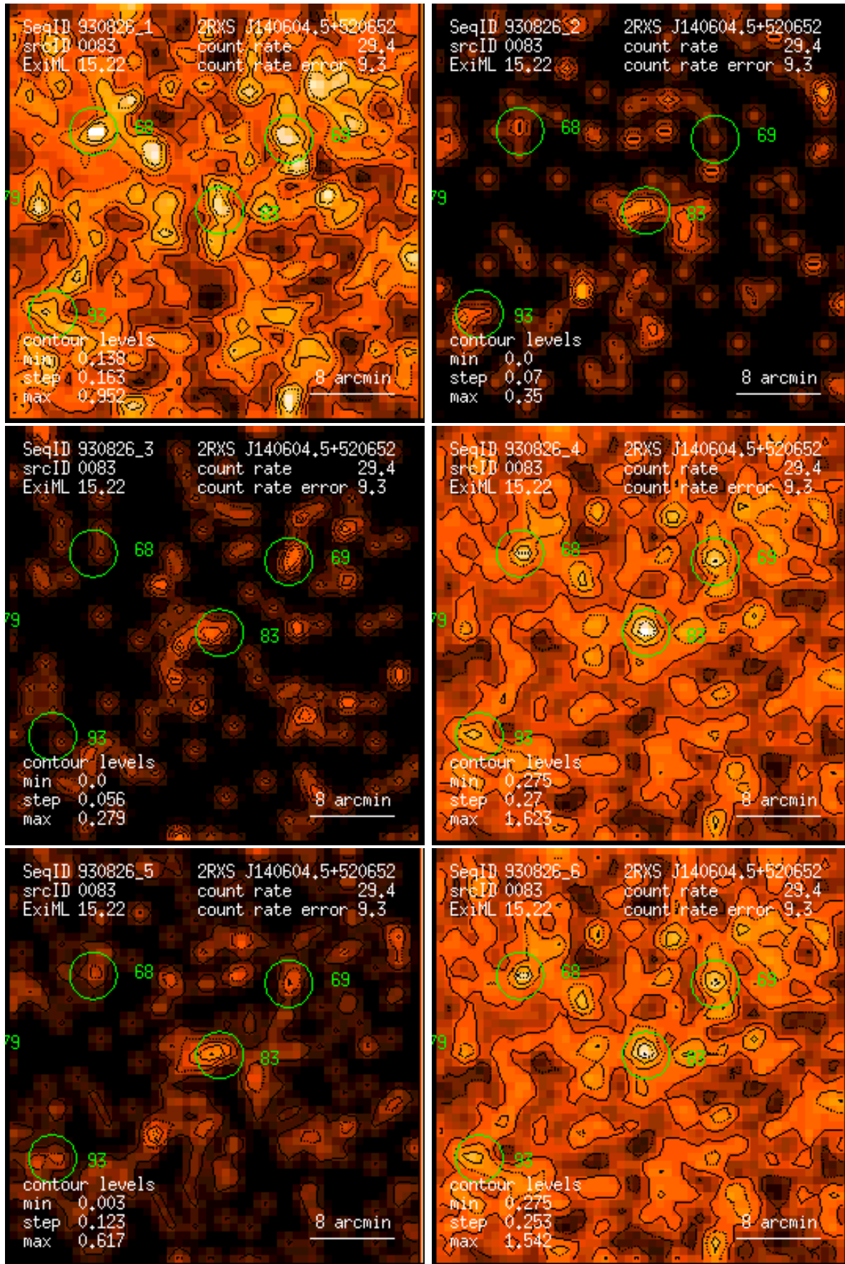
Figure 83: RASS 930826: detection 0083: band rate images, Gaussian filter: (1) PSPC channels 11 – 41, (2) 52 – 90, (3) 91 – 201, (4) 11 – 235, (5) 52 – 201, (6) 11 – 201. Broad band rates in counts/ks. Band rate contour levels in counts/ks/arcmin 2 .
