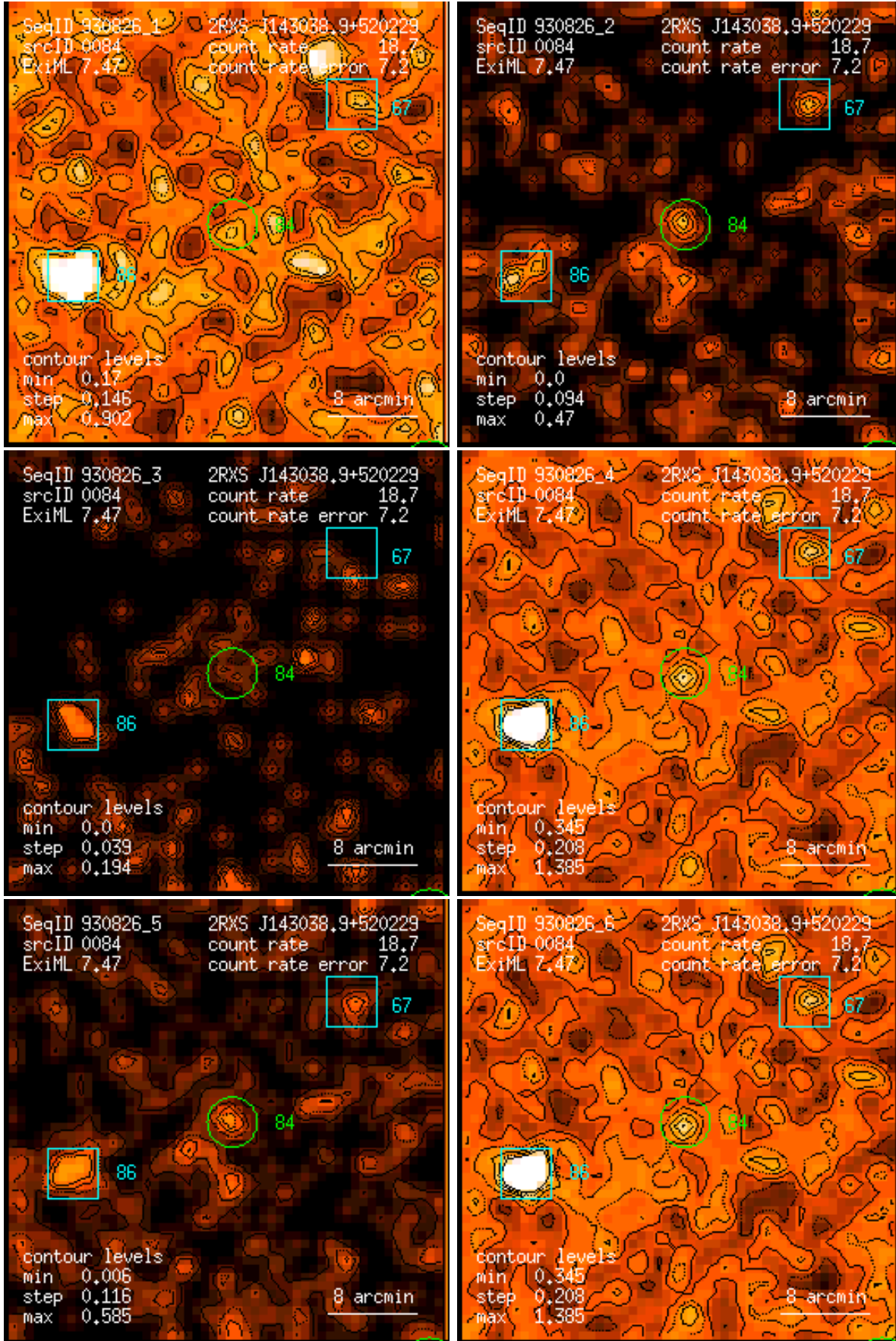
Figure 84: RASS 930826: detection 0084: band rate images, Gaussian filter: (1) PSPC channels 11 – 41, (2) 52 – 90, (3) 91 – 201, (4) 11 – 235, (5) 52 – 201, (6) 11 – 201. Broad band rates in counts/ks. Band rate contour levels in counts/ks/arcmin 2 .
