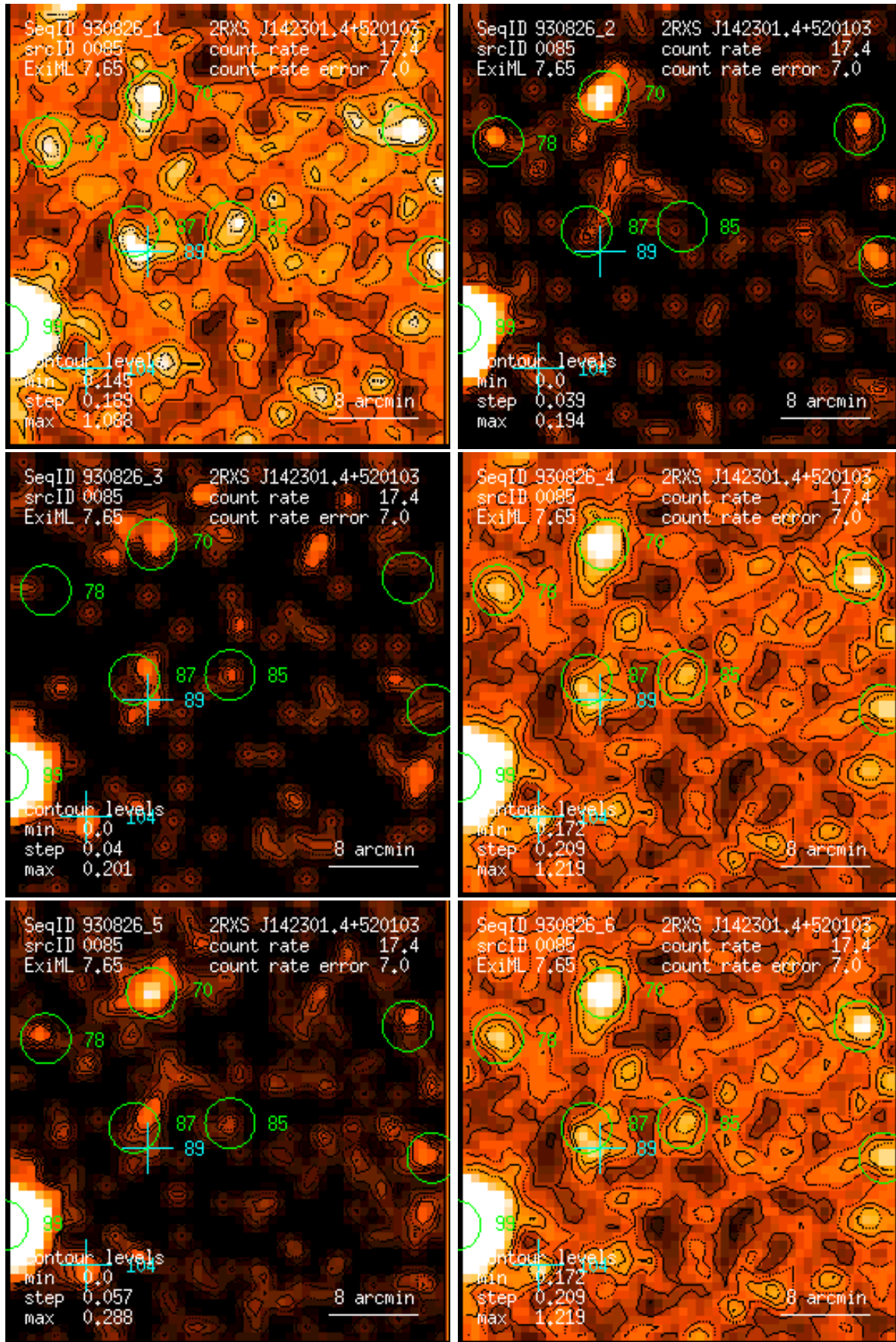
Figure 85: RASS 930826: detection 0085: band rate images, Gaussian filter: (1) PSPC channels 11 – 41, (2) 52 – 90, (3) 91 – 201, (4) 11 – 235, (5) 52 – 201, (6) 11 – 201. Broad band rates in counts/ks. Band rate contour levels in counts/ks/arcmin 2 .
