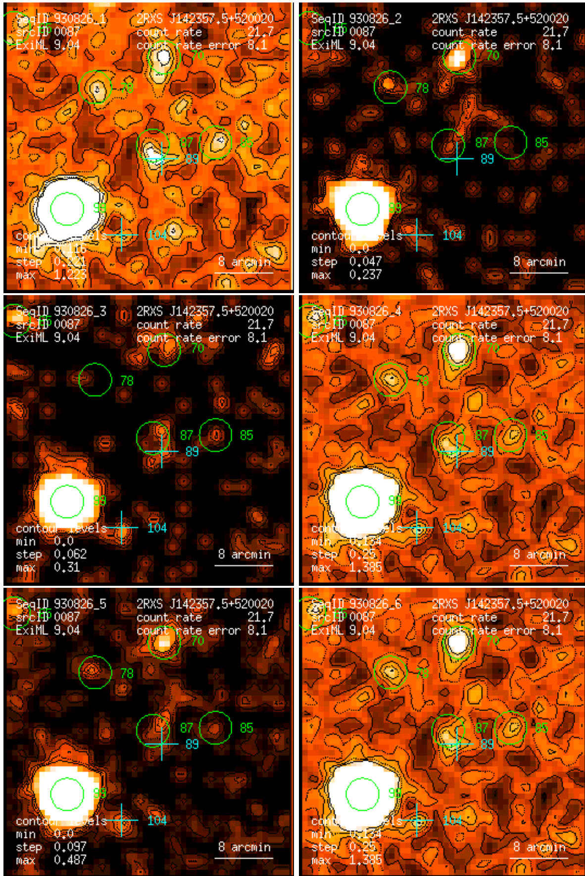
Figure 87: RASS 930826: detection 0087: band rate images, Gaussian filter: (1) PSPC channels 11 – 41, (2) 52 – 90, (3) 91 – 201, (4) 11 – 235, (5) 52 – 201, (6) 11 – 201. Broad band rates in counts/ks. Band rate contour levels in counts/ks/arcmin 2 .
