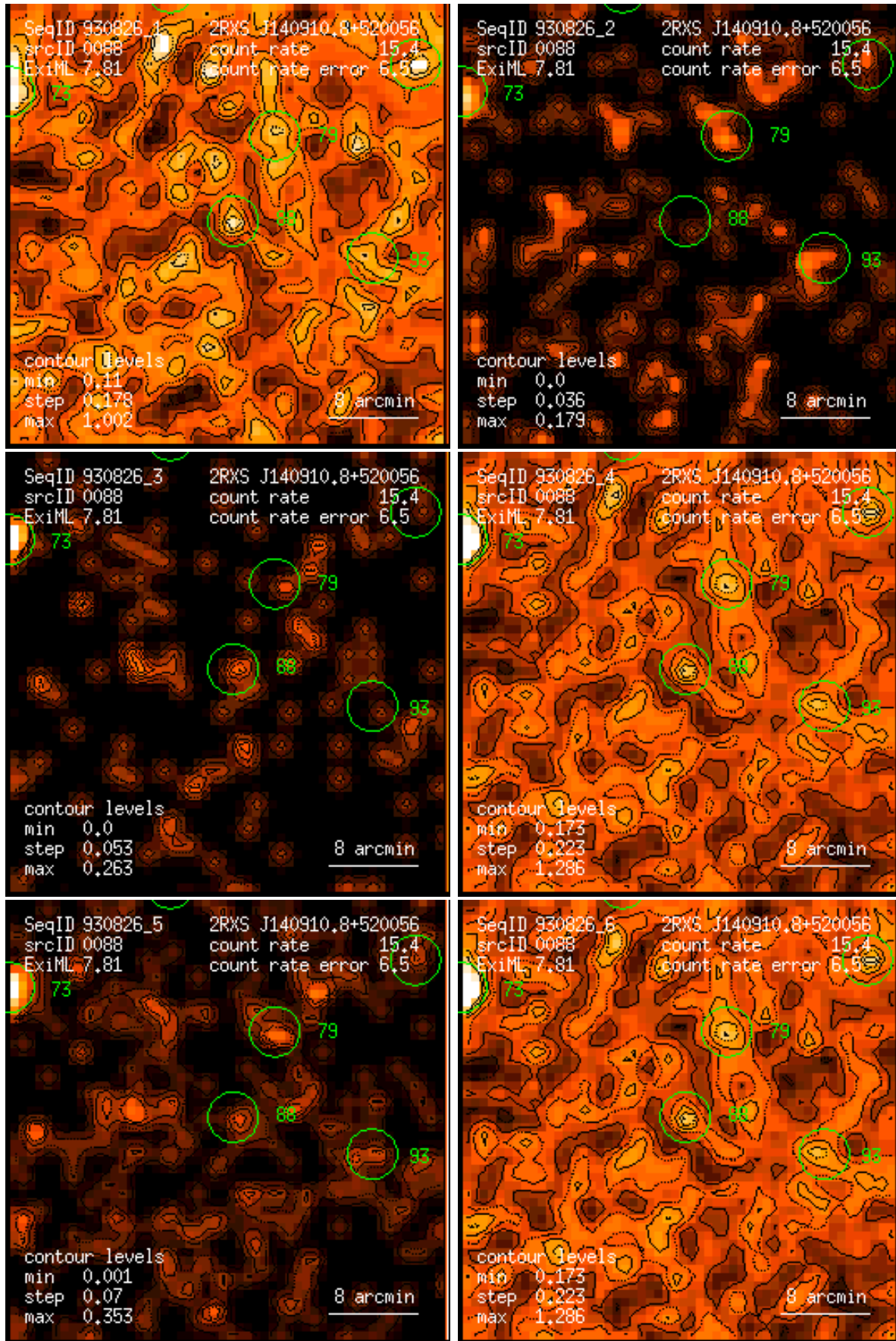
Figure 88: RASS 930826: detection 0088: band rate images, Gaussian filter: (1) PSPC channels 11 – 41, (2) 52 – 90, (3) 91 – 201, (4) 11 – 235, (5) 52 – 201, (6) 11 – 201. Broad band rates in counts/ks. Band rate contour levels in counts/ks/arcmin 2 .
