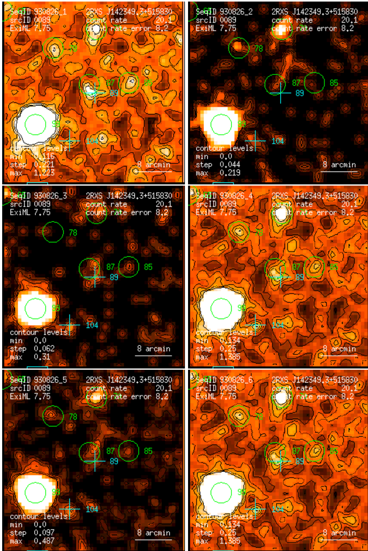
Figure 89: RASS 930826: detection 0089: band rate images, Gaussian filter: (1) PSPC channels 11 – 41, (2) 52 – 90, (3) 91 – 201, (4) 11 – 235, (5) 52 – 201, (6) 11 – 201. Broad band rates in counts/ks. Band rate contour levels in counts/ks/arcmin 2 .
