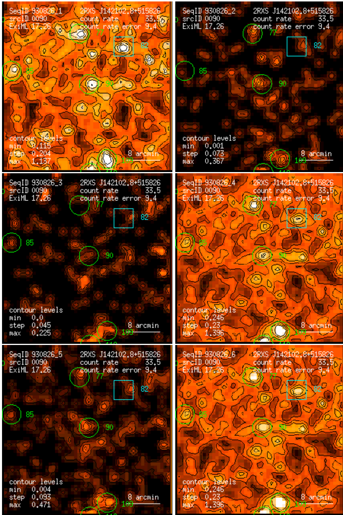
Figure 90: RASS 930826: detection 0090: band rate images, Gaussian filter: (1) PSPC channels 11 – 41, (2) 52 – 90, (3) 91 – 201, (4) 11 – 235, (5) 52 – 201, (6) 11 – 201. Broad band rates in counts/ks. Band rate contour levels in counts/ks/arcmin 2 .
