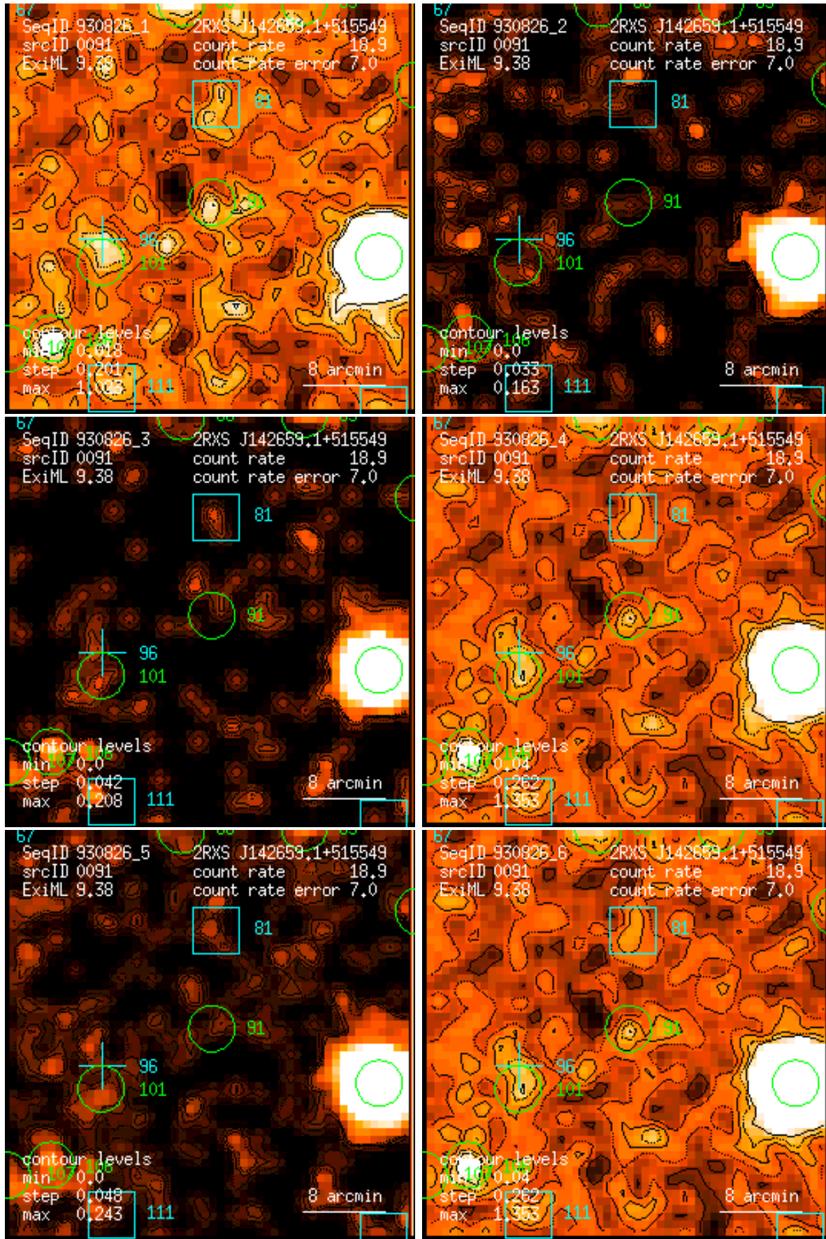
Figure 91: RASS 930826: detection 0091: band rate images, Gaussian filter: (1) PSPC channels 11 – 41, (2) 52 – 90, (3) 91 – 201, (4) 11 – 235, (5) 52 – 201, (6) 11 – 201. Broad band rates in counts/ks. Band rate contour levels in counts/ks/arcmin 2 .
