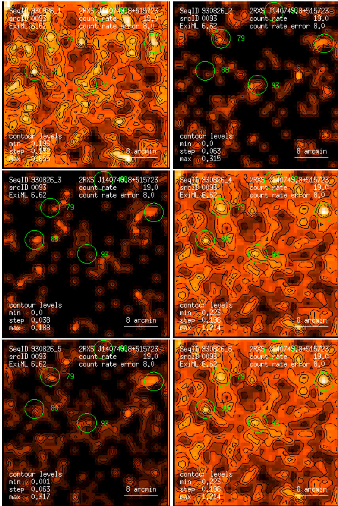
Figure 93: RASS 930826: detection 0093: band rate images, Gaussian filter: (1) PSPC channels 11 – 41, (2) 52 – 90, (3) 91 – 201, (4) 11 – 235, (5) 52 – 201, (6) 11 – 201. Broad band rates in counts/ks. Band rate contour levels in counts/ks/arcmin 2 .
