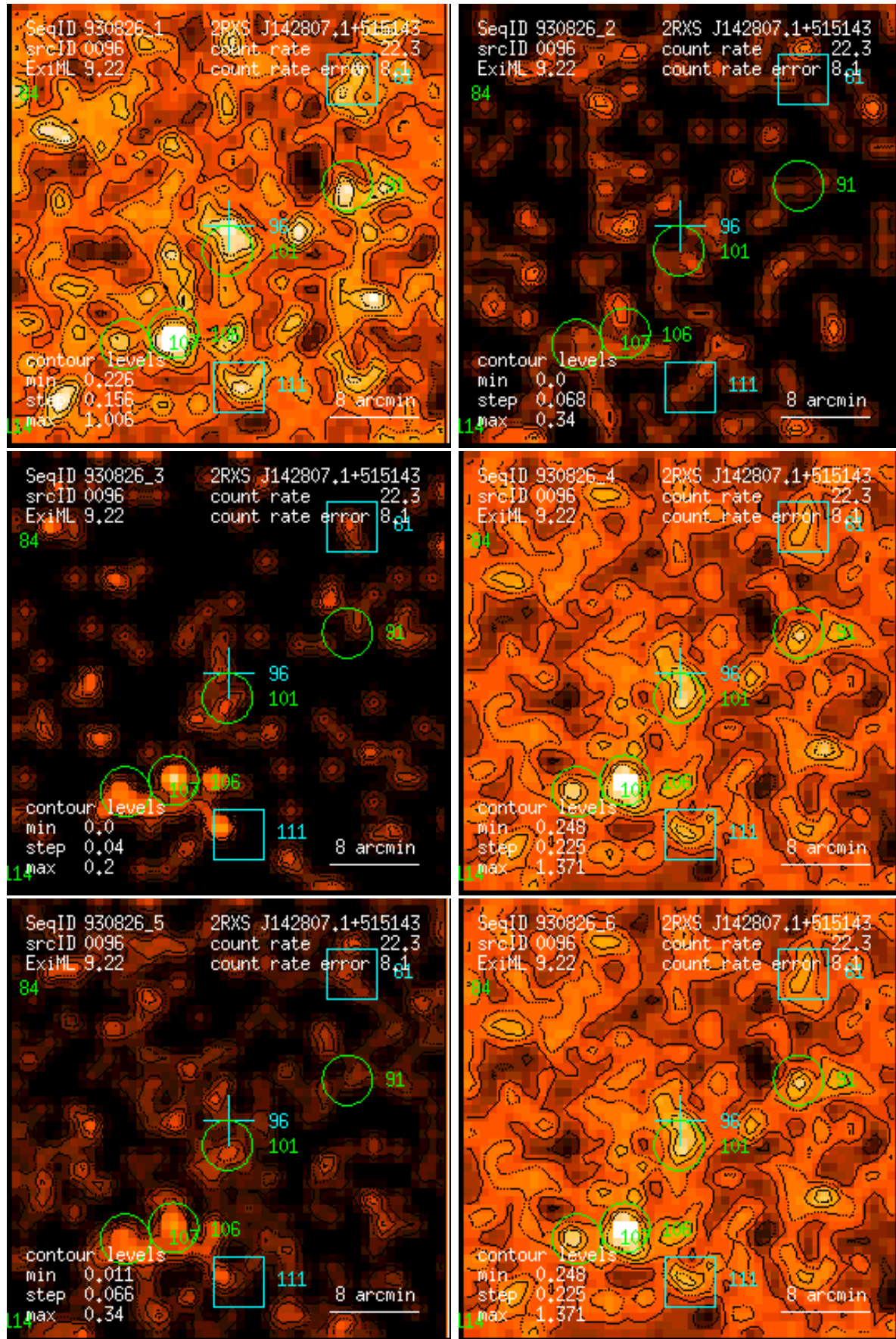
Figure 96: RASS 930826: detection 0096: band rate images, Gaussian filter: (1) PSPC channels 11 – 41, (2) 52 – 90, (3) 91 – 201, (4) 11 – 235, (5) 52 – 201, (6) 11 – 201. Broad band rates in counts/ks. Band rate contour levels in counts/ks/arcmin 2 .
