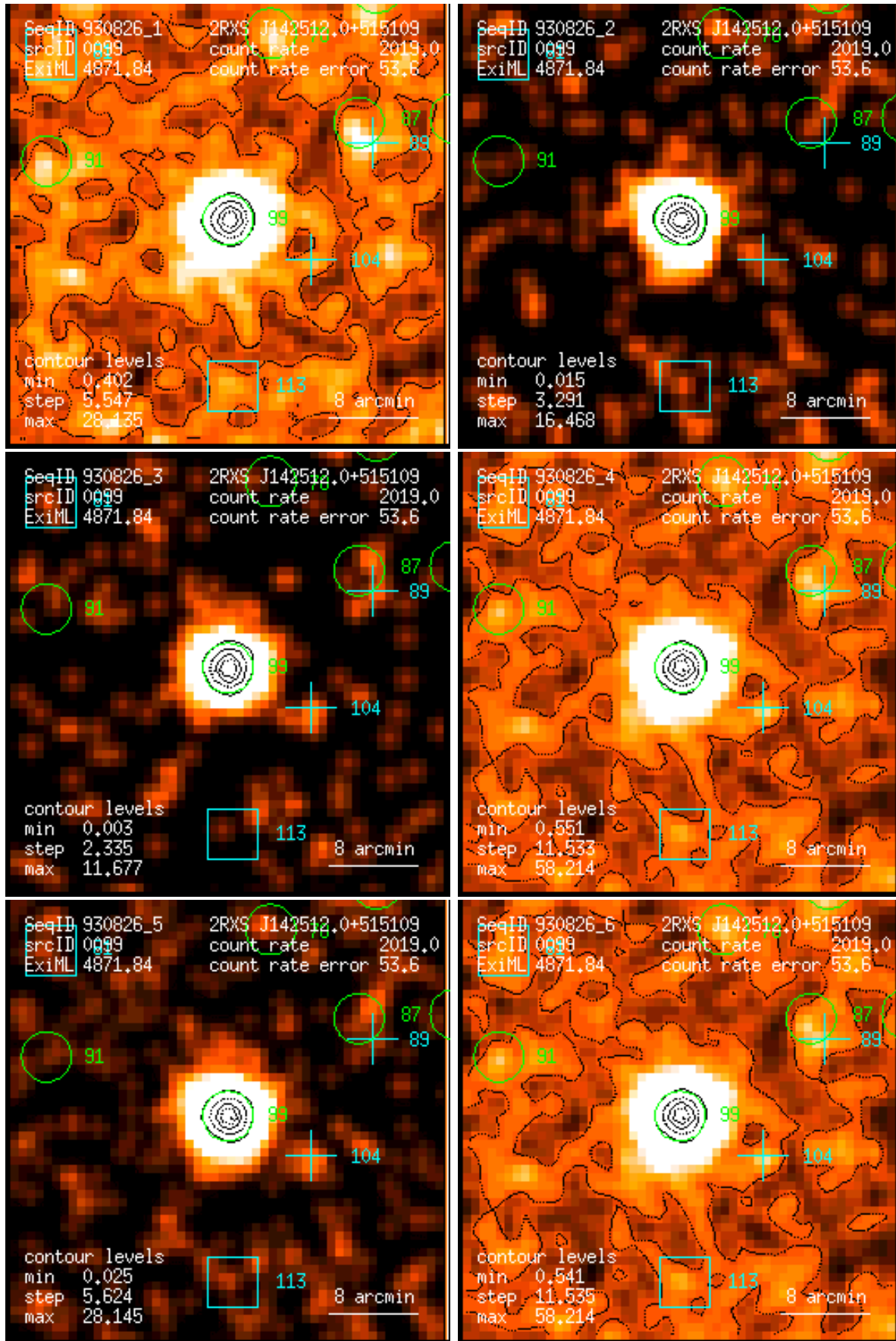
Figure 99: RASS 930826: detection 0099: band rate images, Gaussian filter: (1) PSPC channels 11 – 41, (2) 52 – 90, (3) 91 – 201, (4) 11 – 235, (5) 52 – 201, (6) 11 – 201. Broad band rates in counts/ks. Band rate contour levels in counts/ks/arcmin 2 .
