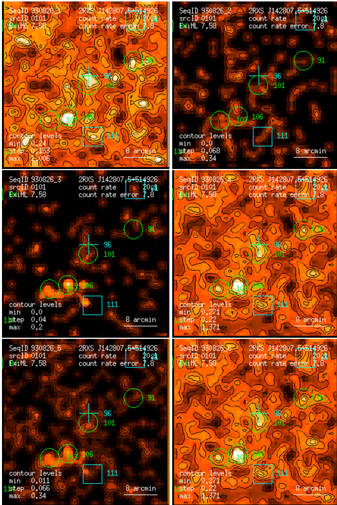
Figure 101: RASS 930826: detection 0101: band rate images, Gaussian filter: (1) PSPC channels 11 – 41, (2) 52 – 90, (3) 91 – 201, (4) 11 – 235, (5) 52 – 201, (6) 11 – 201. Broad band rates in counts/ks. Band rate contour levels in counts/ks/arcmin 2 .
