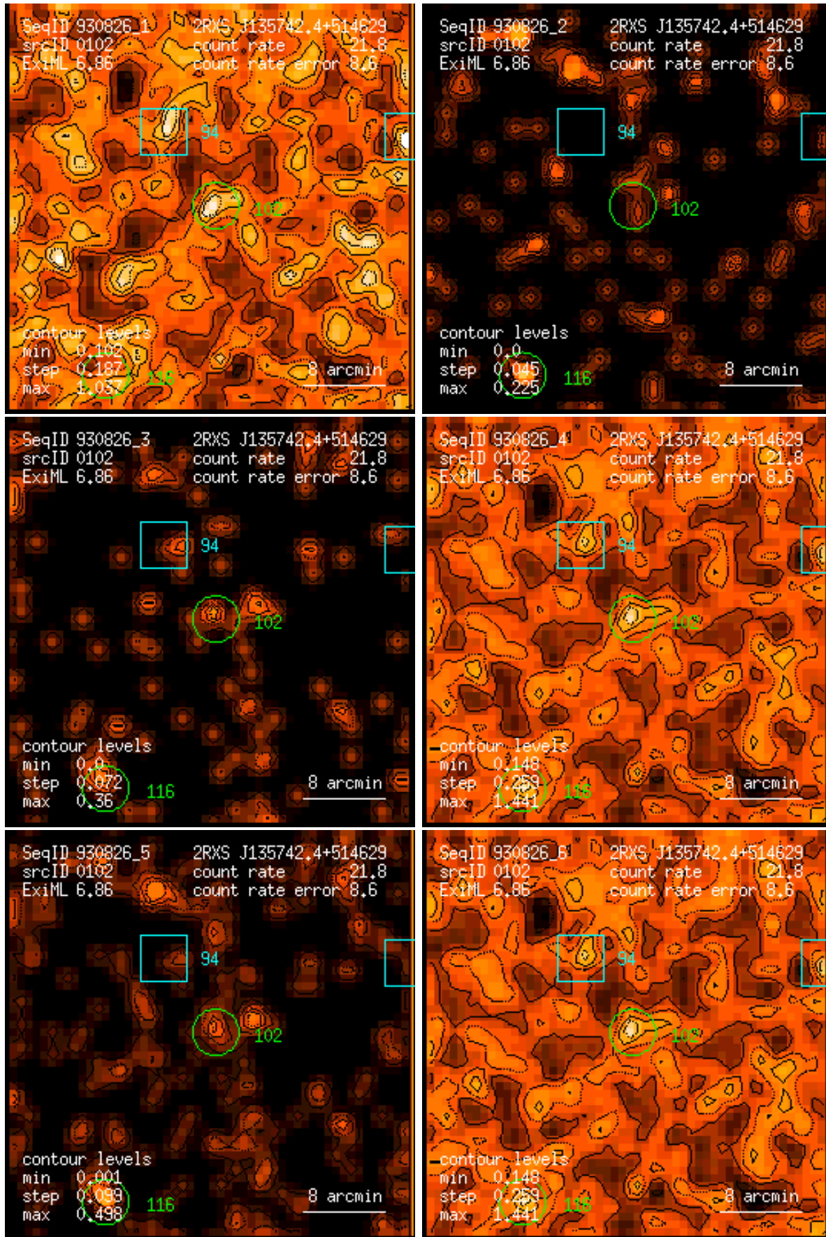
Figure 102: RASS 930826: detection 0102: band rate images, Gaussian filter: (1) PSPC channels 11 – 41, (2) 52 – 90, (3) 91 – 201, (4) 11 – 235, (5) 52 – 201, (6) 11 – 201. Broad band rates in counts/ks. Band rate contour levels in counts/ks/arcmin 2 .
