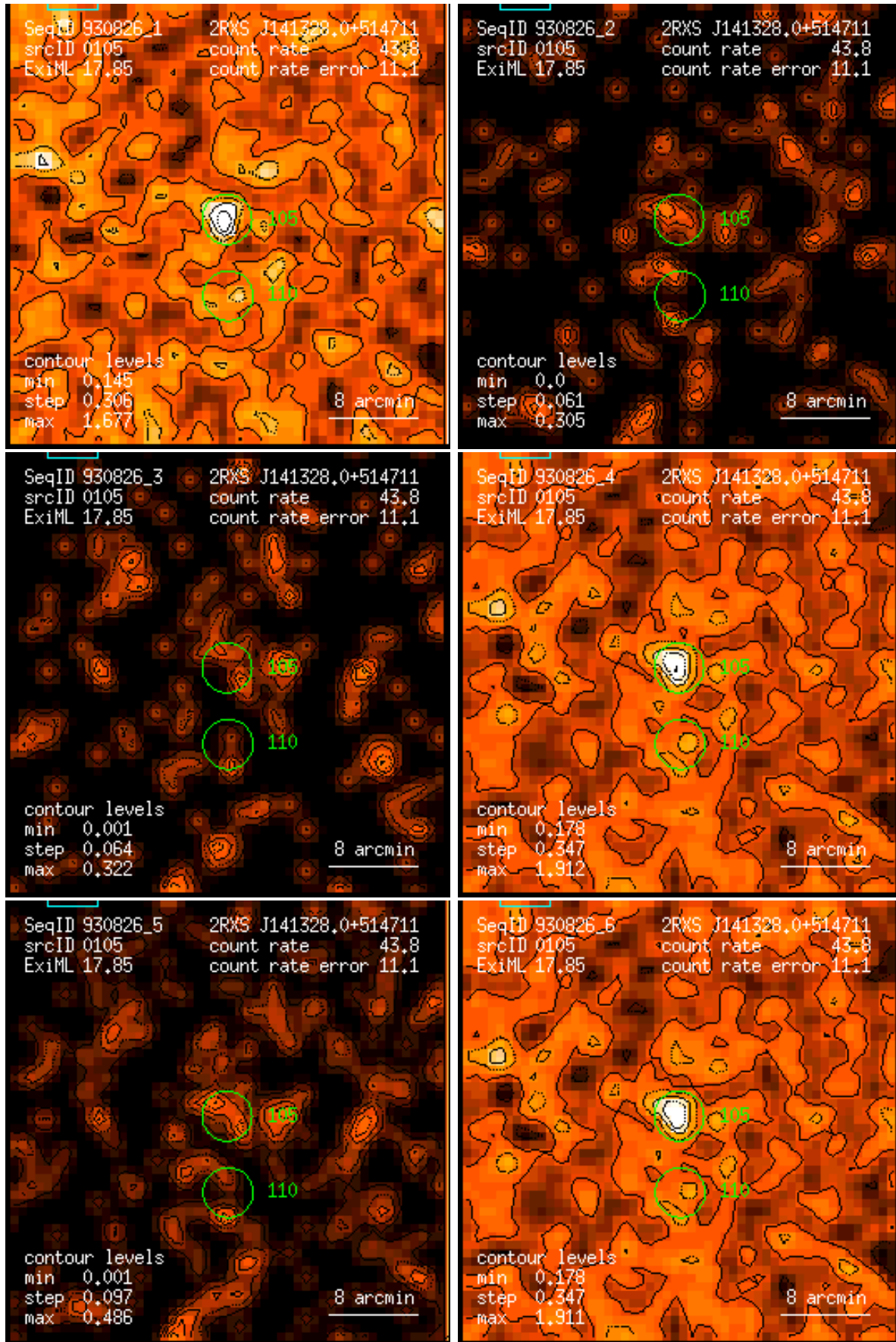
Figure 105: RASS 930826: detection 0105: band rate images, Gaussian filter: (1) PSPC channels 11 – 41, (2) 52 – 90, (3) 91 – 201, (4) 11 – 235, (5) 52 – 201, (6) 11 – 201. Broad band rates in counts/ks. Band rate contour levels in counts/ks/arcmin 2 .
