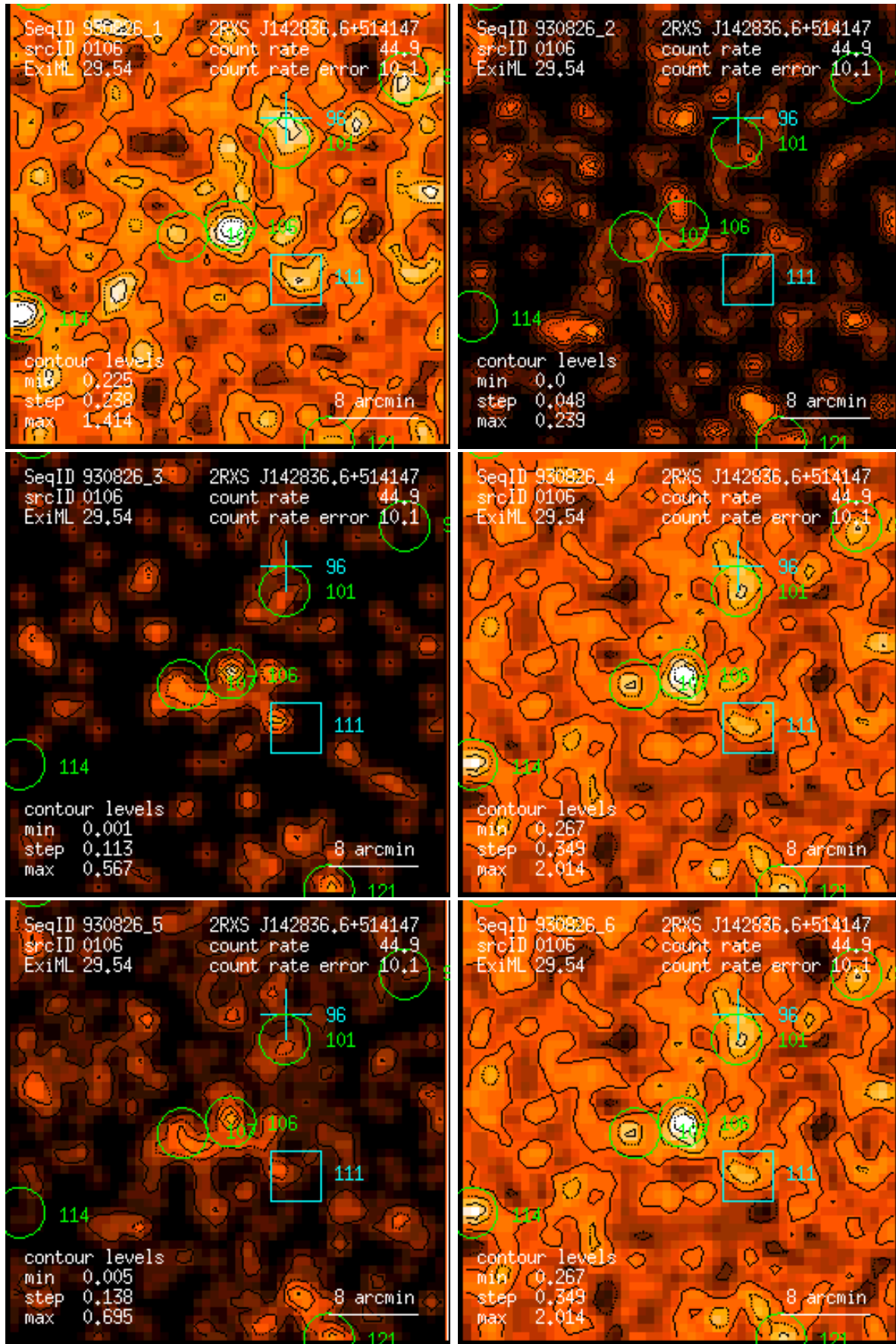
Figure 106: RASS 930826: detection 0106: band rate images, Gaussian filter: (1) PSPC channels 11 – 41, (2) 52 – 90, (3) 91 – 201, (4) 11 – 235, (5) 52 – 201, (6) 11 – 201. Broad band rates in counts/ks. Band rate contour levels in counts/ks/arcmin 2 .
