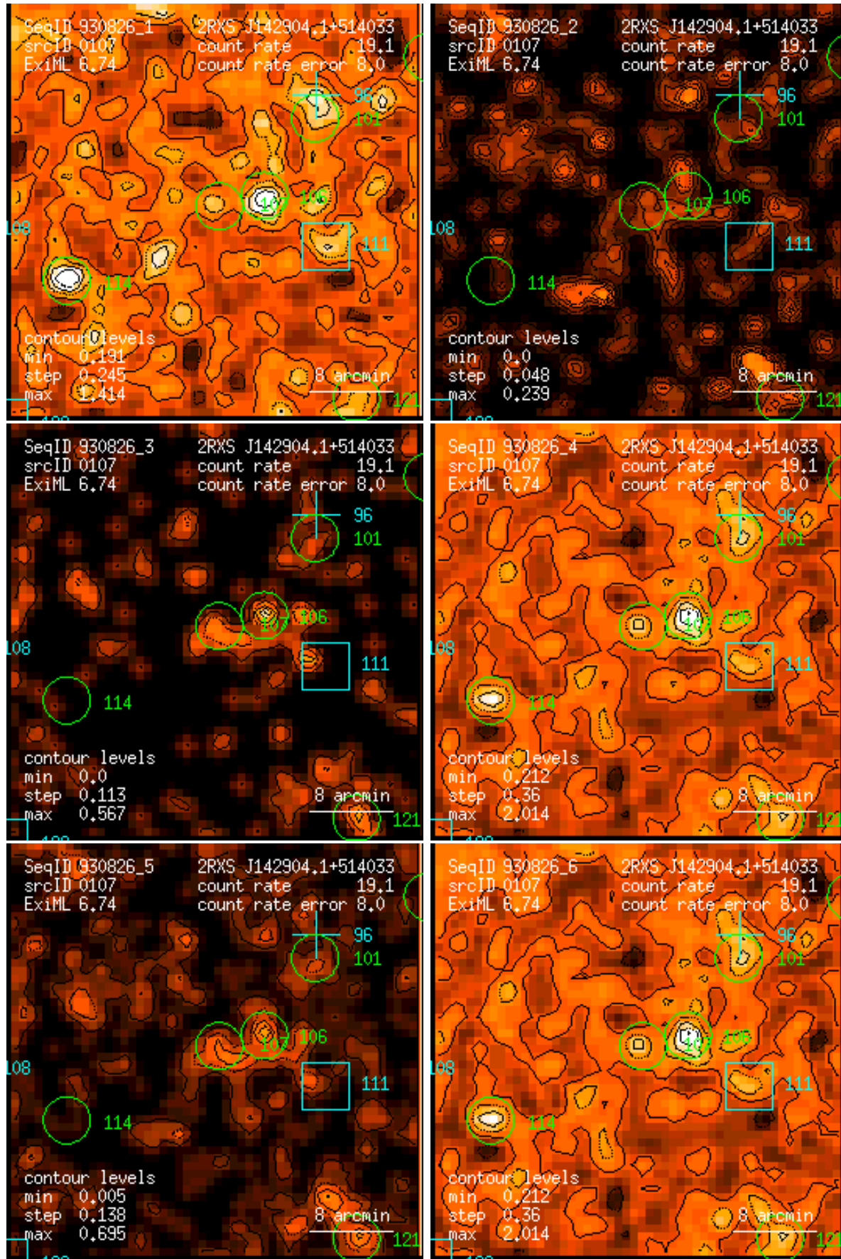
Figure 107: RASS 930826: detection 0107: band rate images, Gaussian filter: (1) PSPC channels 11 – 41, (2) 52 – 90, (3) 91 – 201, (4) 11 – 235, (5) 52 – 201, (6) 11 – 201. Broad band rates in counts/ks. Band rate contour levels in counts/ks/arcmin 2 .
