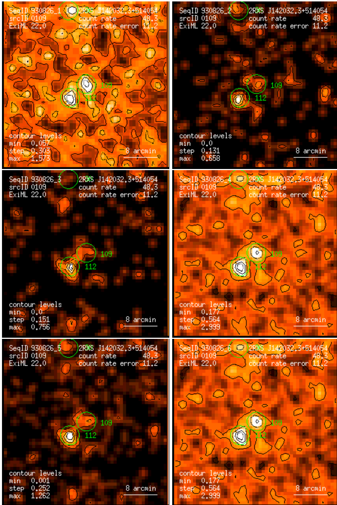
Figure 109: RASS 930826: detection 0109: band rate images, Gaussian filter: (1) PSPC channels 11 – 41, (2) 52 – 90, (3) 91 – 201, (4) 11 – 235, (5) 52 – 201, (6) 11 – 201. Broad band rates in counts/ks. Band rate contour levels in counts/ks/arcmin 2 .
