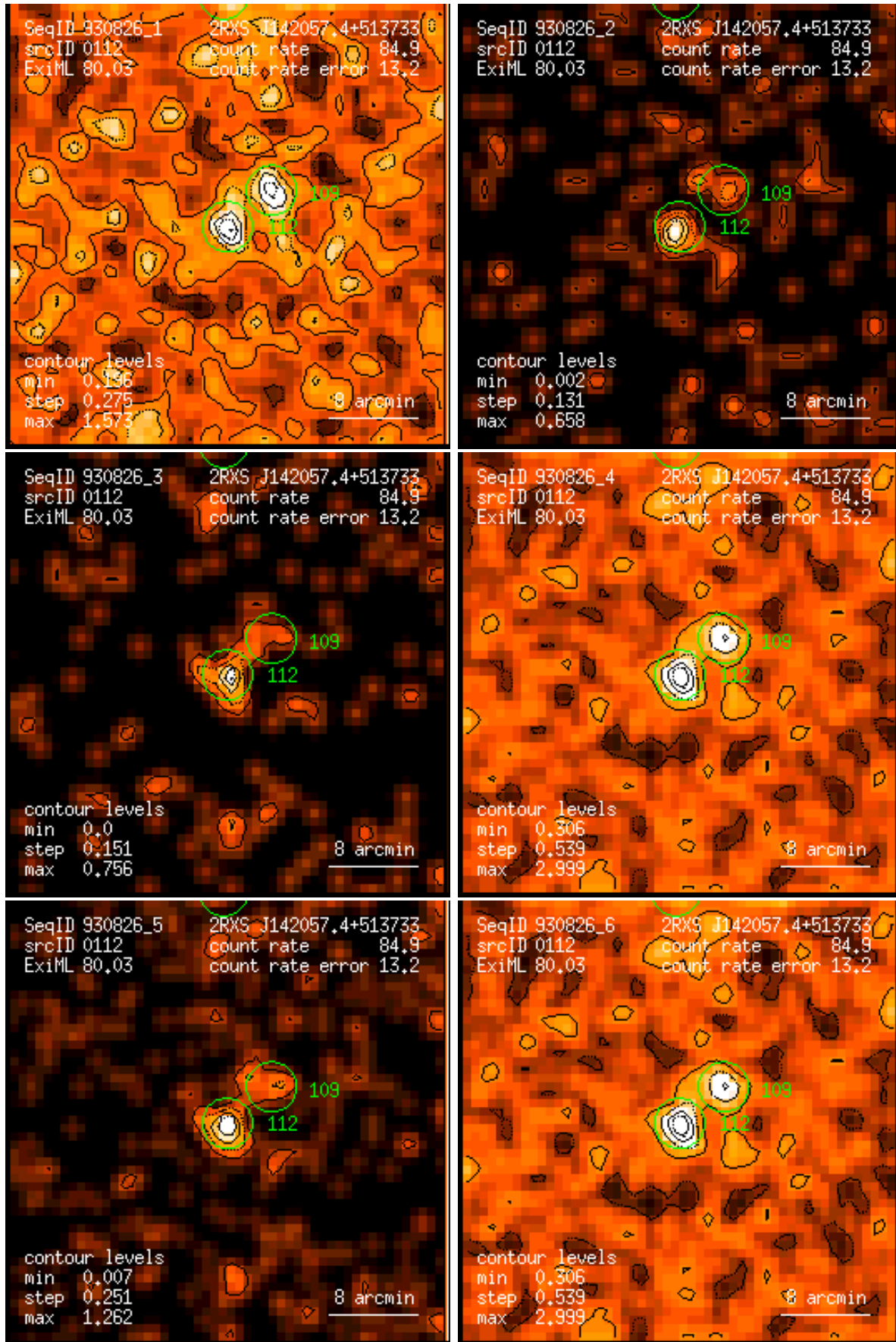
Figure 112: RASS 930826: detection 0112: band rate images, Gaussian filter: (1) PSPC channels 11 – 41, (2) 52 – 90, (3) 91 – 201, (4) 11 – 235, (5) 52 – 201, (6) 11 – 201. Broad band rates in counts/ks. Band rate contour levels in counts/ks/arcmin 2 .
