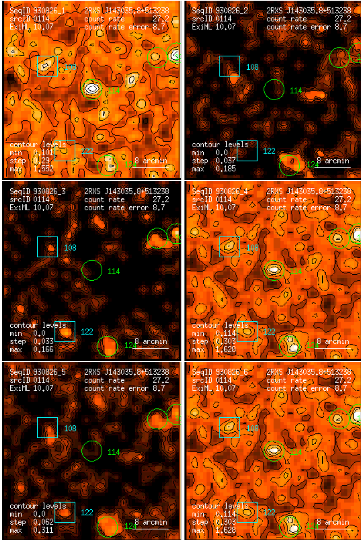
Figure 114: RASS 930826: detection 0114: band rate images, Gaussian filter: (1) PSPC channels 11 – 41, (2) 52 – 90, (3) 91 – 201, (4) 11 – 235, (5) 52 – 201, (6) 11 – 201. Broad band rates in counts/ks. Band rate contour levels in counts/ks/arcmin 2 .
