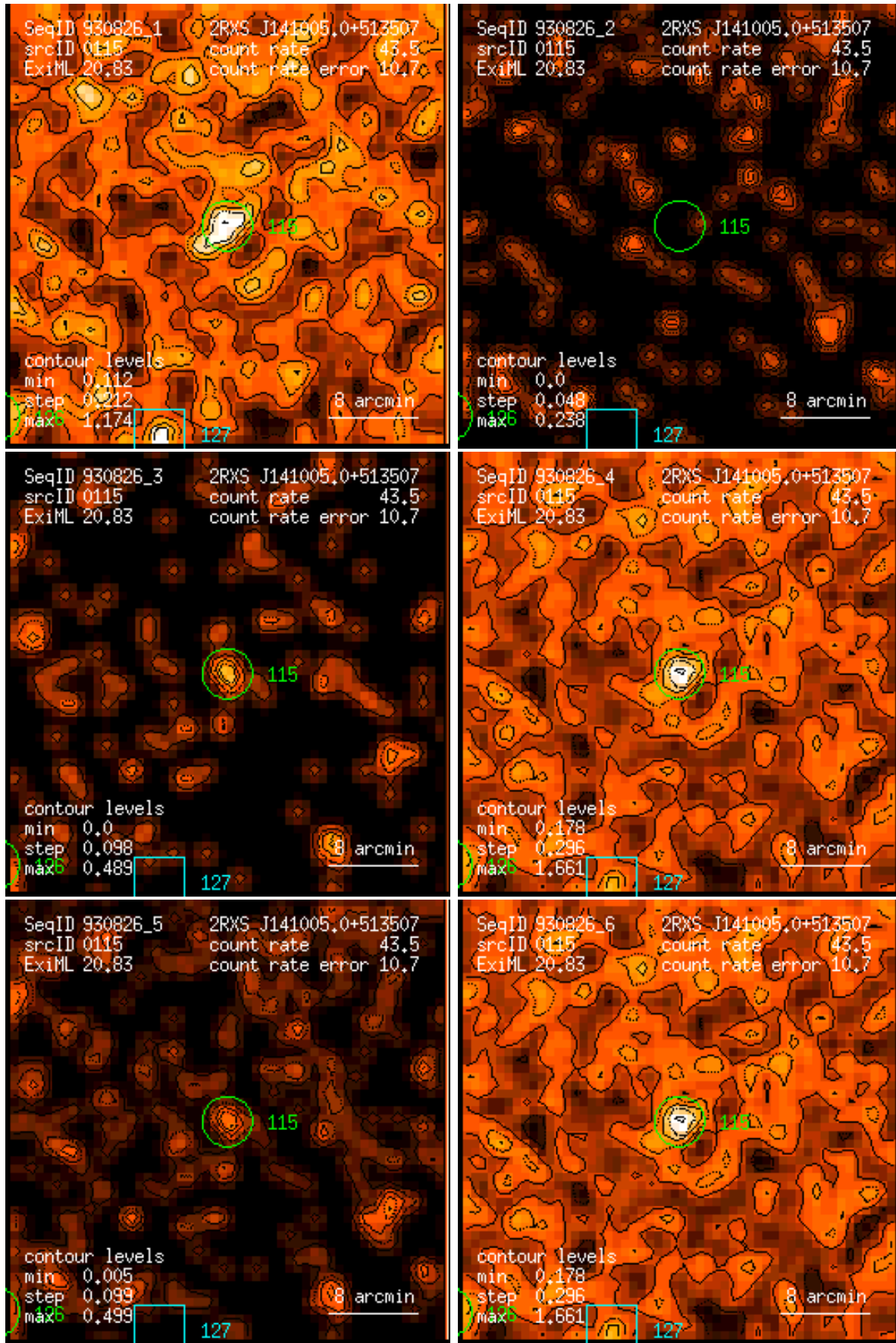
Figure 115: RASS 930826: detection 0115: band rate images, Gaussian filter: (1) PSPC channels 11 – 41, (2) 52 – 90, (3) 91 – 201, (4) 11 – 235, (5) 52 – 201, (6) 11 – 201. Broad band rates in counts/ks. Band rate contour levels in counts/ks/arcmin 2 .
