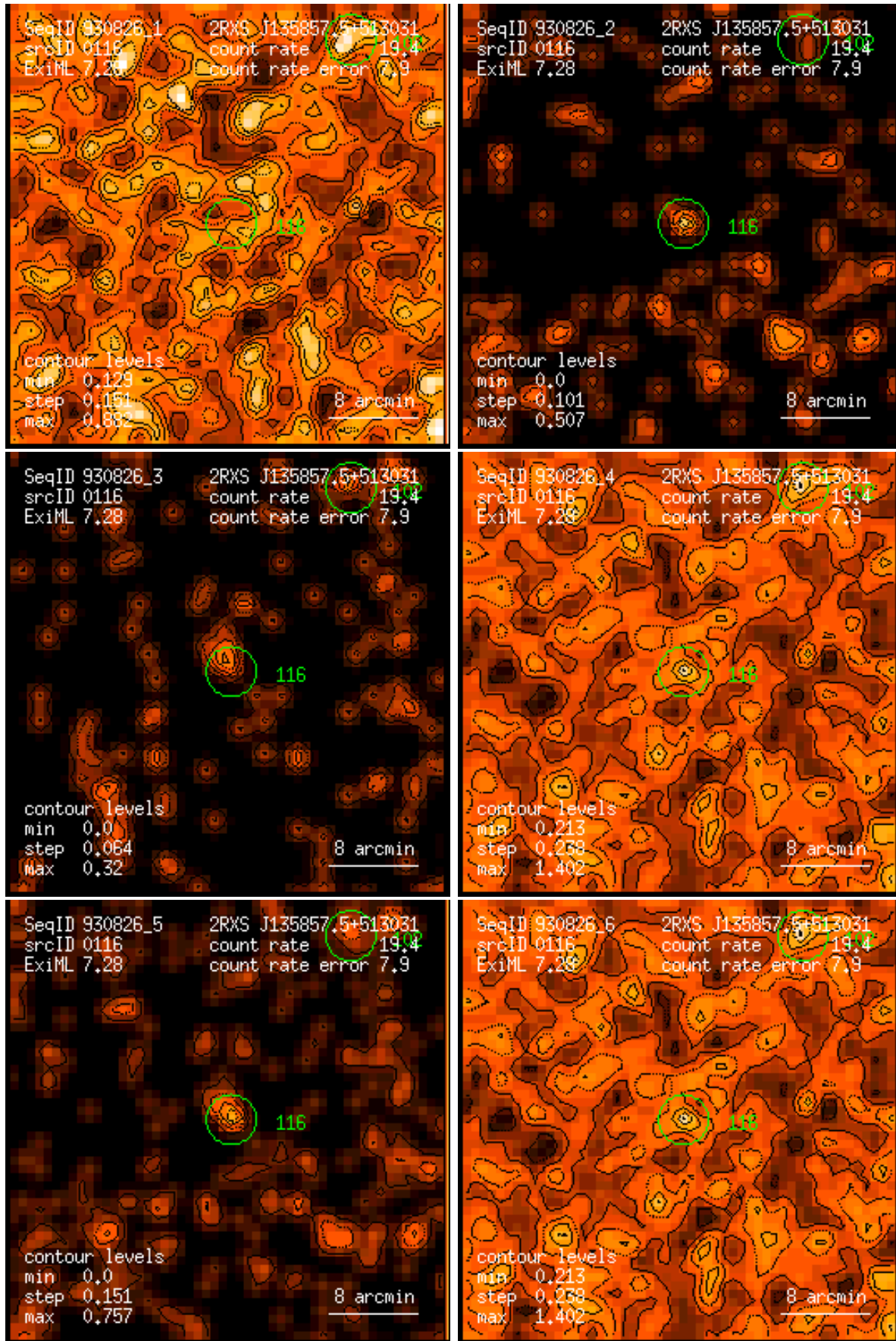
Figure 116: RASS 930826: detection 0116: band rate images, Gaussian filter: (1) PSPC channels 11 – 41, (2) 52 – 90, (3) 91 – 201, (4) 11 – 235, (5) 52 – 201, (6) 11 – 201. Broad band rates in counts/ks. Band rate contour levels in counts/ks/arcmin 2 .
