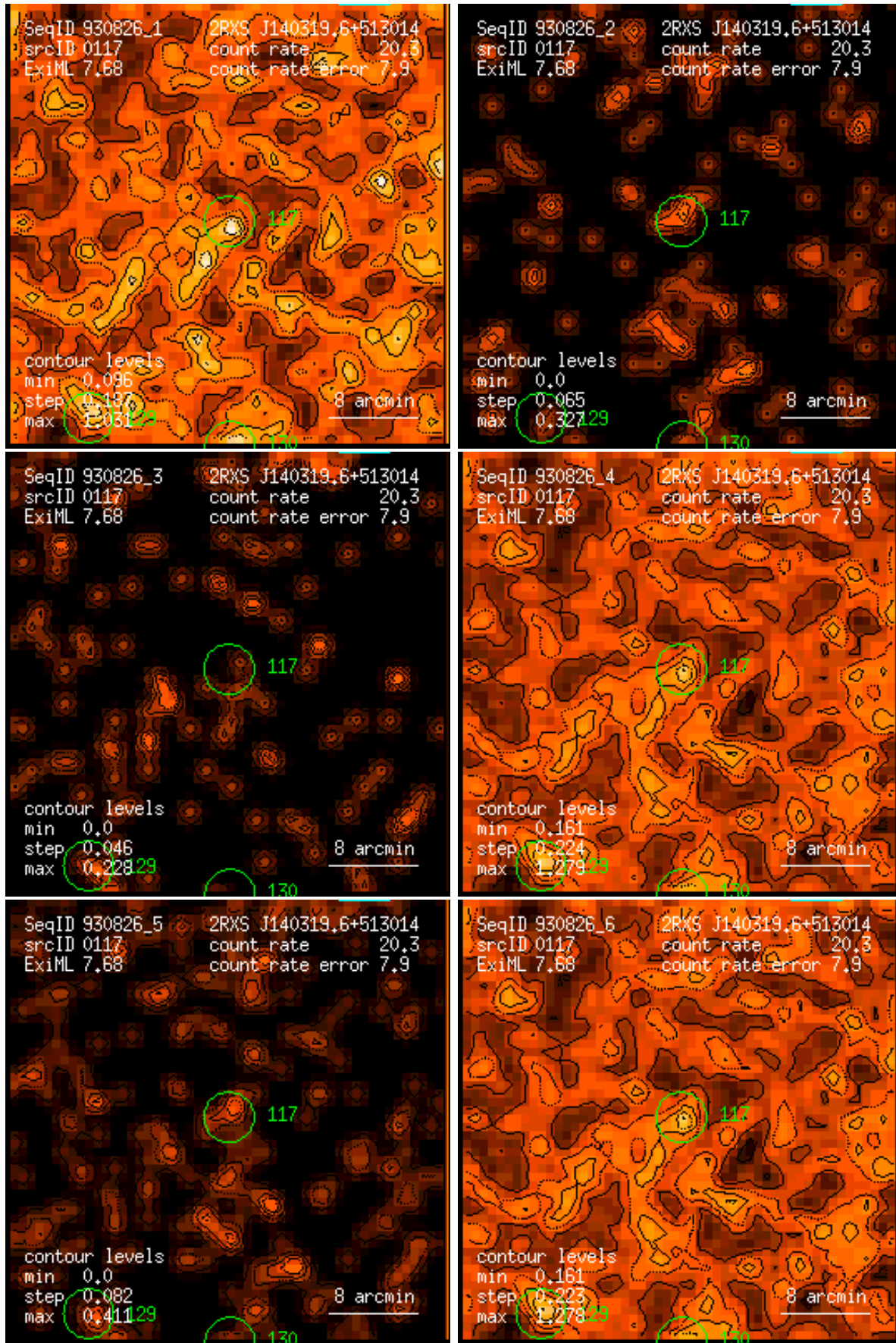
Figure 117: RASS 930826: detection 0117: band rate images, Gaussian filter: (1) PSPC channels 11 – 41, (2) 52 – 90, (3) 91 – 201, (4) 11 – 235, (5) 52 – 201, (6) 11 – 201. Broad band rates in counts/ks. Band rate contour levels in counts/ks/arcmin 2 .
