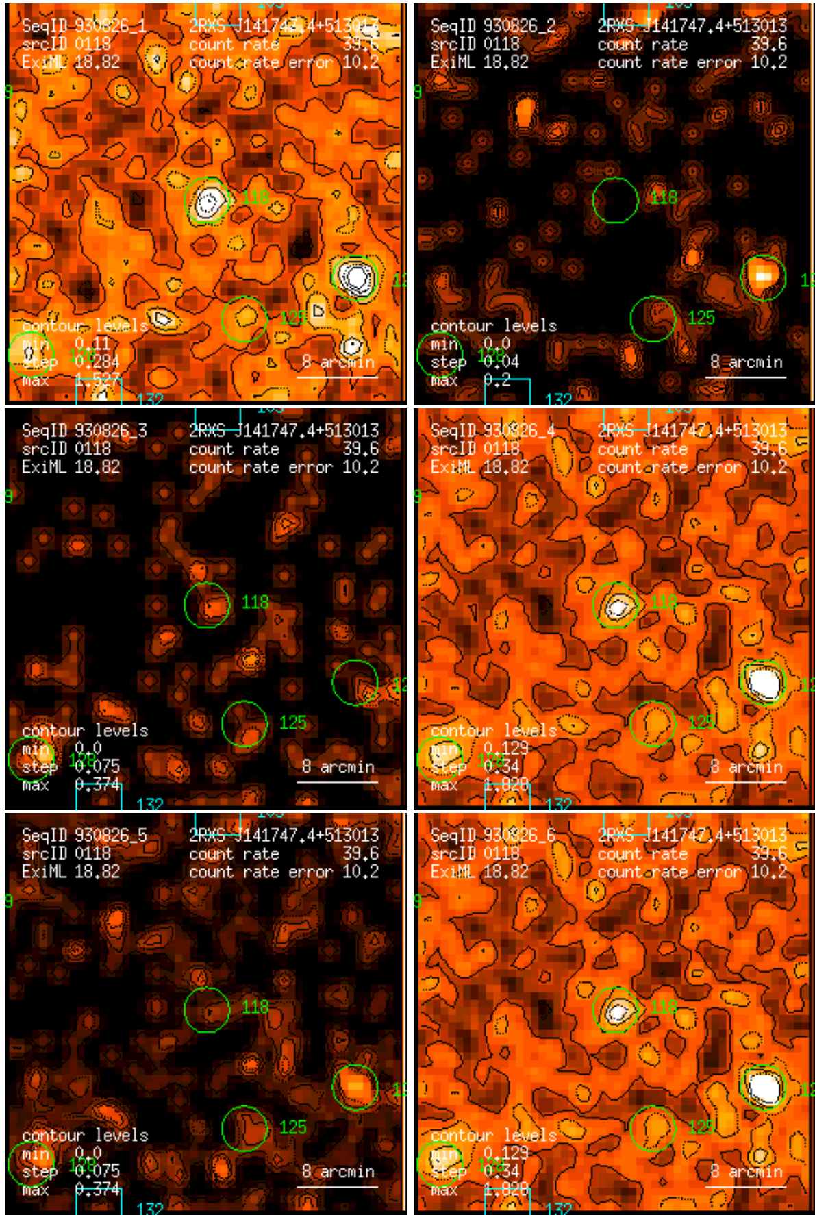
Figure 118: RASS 930826: detection 0118: band rate images, Gaussian filter: (1) PSPC channels 11 – 41, (2) 52 – 90, (3) 91 – 201, (4) 11 – 235, (5) 52 – 201, (6) 11 – 201. Broad band rates in counts/ks. Band rate contour levels in counts/ks/arcmin 2 .
