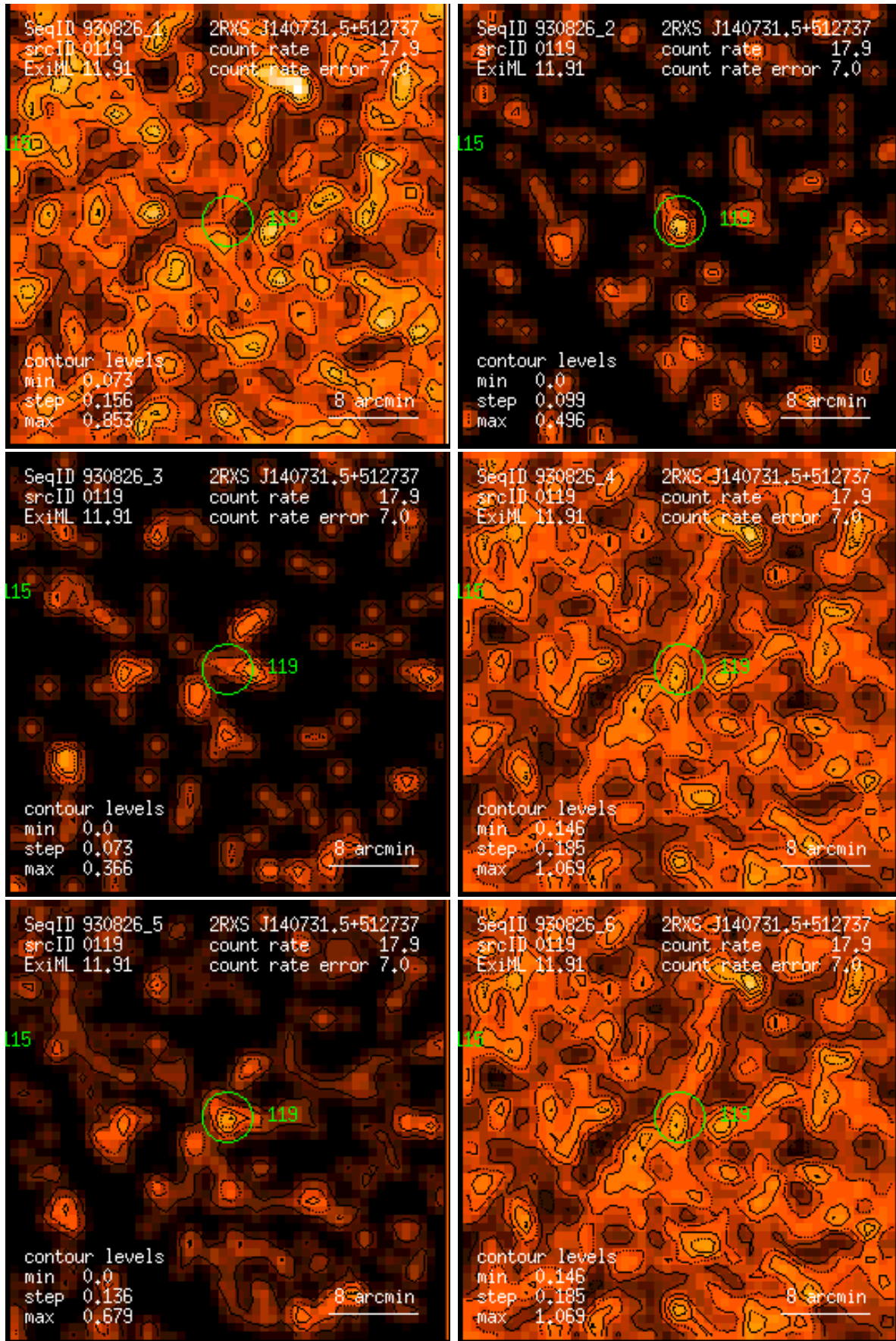
Figure 119: RASS 930826: detection 0119: band rate images, Gaussian filter: (1) PSPC channels 11 – 41, (2) 52 – 90, (3) 91 – 201, (4) 11 – 235, (5) 52 – 201, (6) 11 – 201. Broad band rates in counts/ks. Band rate contour levels in counts/ks/arcmin 2 .
