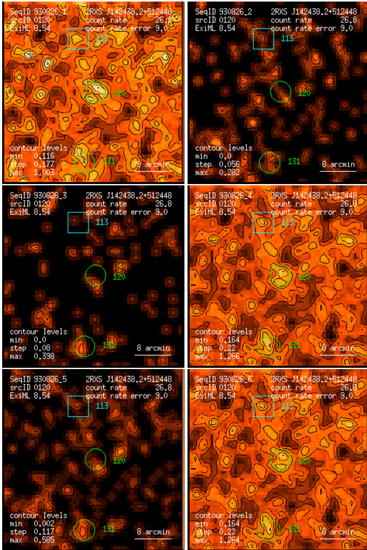
Figure 120: RASS 930826: detection 0120: band rate images, Gaussian filter: (1) PSPC channels 11 – 41, (2) 52 – 90, (3) 91 – 201, (4) 11 – 235, (5) 52 – 201, (6) 11 – 201. Broad band rates in counts/ks. Band rate contour levels in counts/ks/arcmin 2 .
