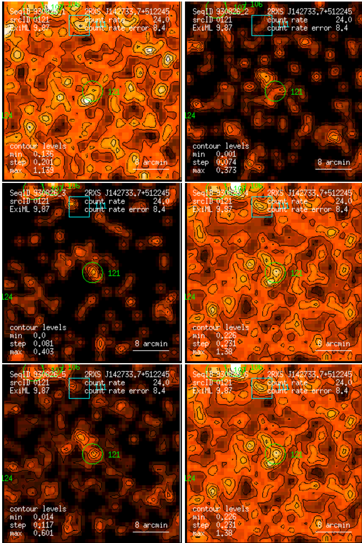
Figure 121: RASS 930826: detection 0121: band rate images, Gaussian filter: (1) PSPC channels 11 – 41, (2) 52 – 90, (3) 91 – 201, (4) 11 – 235, (5) 52 – 201, (6) 11 – 201. Broad band rates in counts/ks. Band rate contour levels in counts/ks/arcmin 2 .
