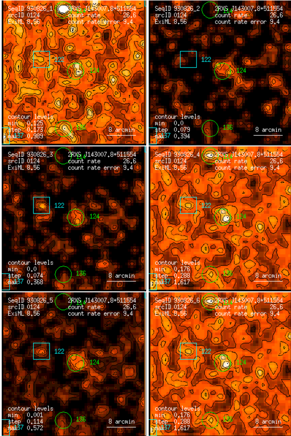
Figure 124: RASS 930826: detection 0124: band rate images, Gaussian filter: (1) PSPC channels 11 – 41, (2) 52 – 90, (3) 91 – 201, (4) 11 – 235, (5) 52 – 201, (6) 11 – 201. Broad band rates in counts/ks. Band rate contour levels in counts/ks/arcmin 2 .
