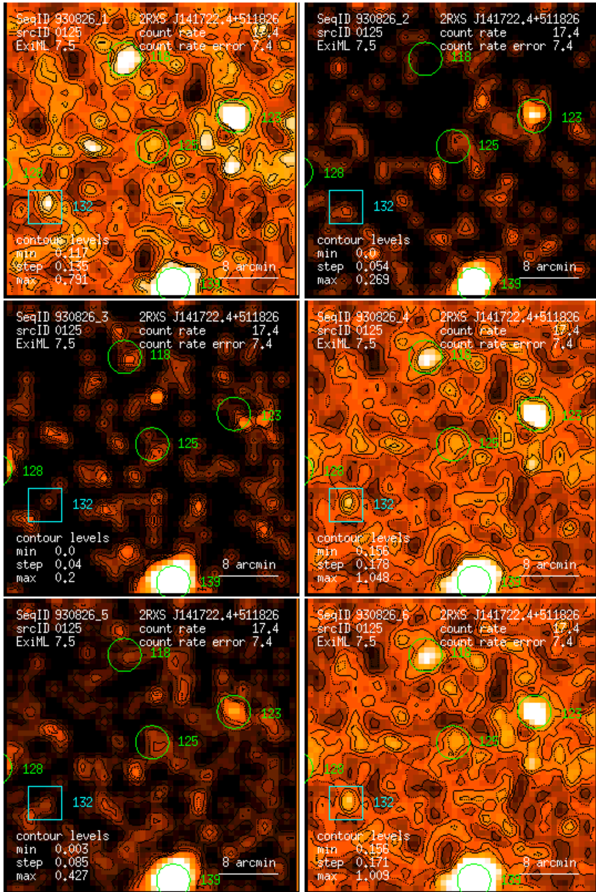
Figure 125: RASS 930826: detection 0125: band rate images, Gaussian filter: (1) PSPC channels 11 – 41, (2) 52 – 90, (3) 91 – 201, (4) 11 – 235, (5) 52 – 201, (6) 11 – 201. Broad band rates in counts/ks. Band rate contour levels in counts/ks/arcmin 2 .
