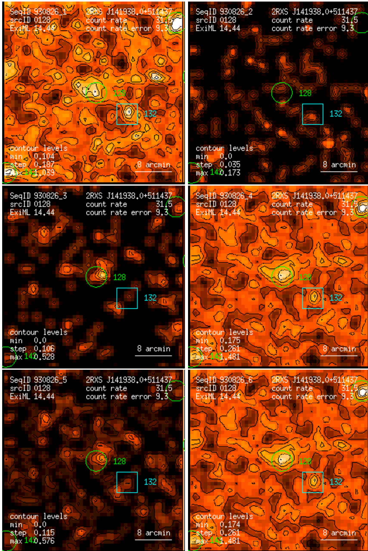
Figure 128: RASS 930826: detection 0128: band rate images, Gaussian filter: (1) PSPC channels 11 – 41, (2) 52 – 90, (3) 91 – 201, (4) 11 – 235, (5) 52 – 201, (6) 11 – 201. Broad band rates in counts/ks. Band rate contour levels in counts/ks/arcmin 2 .
