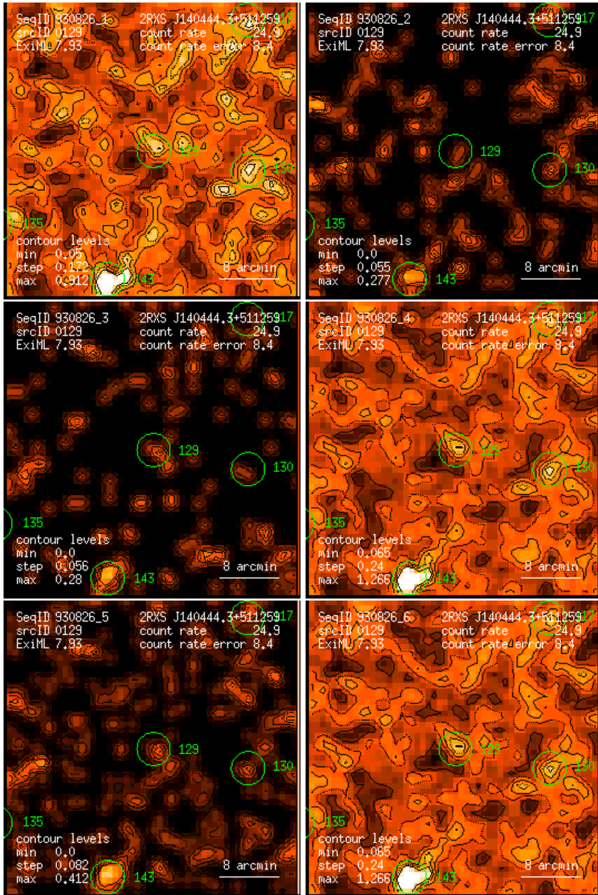
Figure 129: RASS 930826: detection 0129: band rate images, Gaussian filter: (1) PSPC channels 11 – 41, (2) 52 – 90, (3) 91 – 201, (4) 11 – 235, (5) 52 – 201, (6) 11 – 201. Broad band rates in counts/ks. Band rate contour levels in counts/ks/arcmin 2 .
