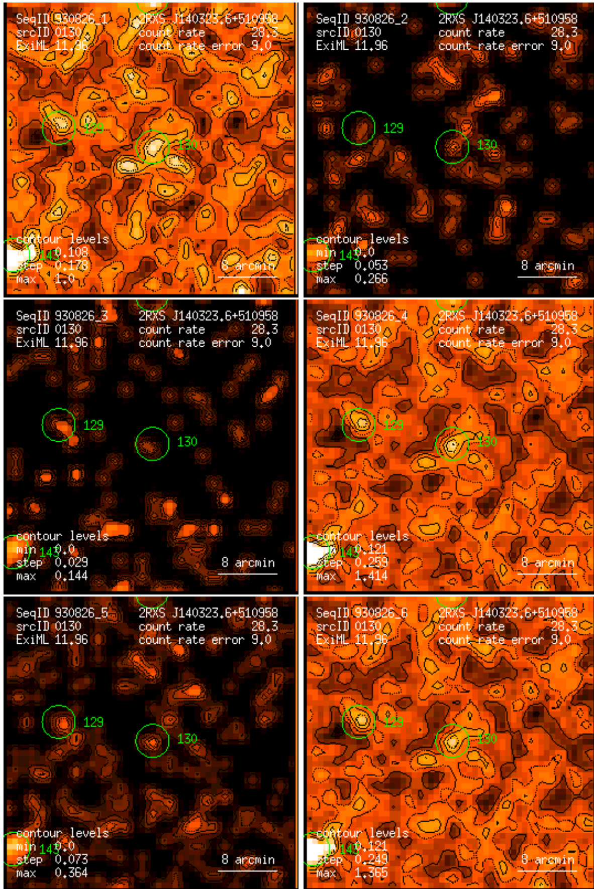
Figure 130: RASS 930826: detection 0130: band rate images, Gaussian filter: (1) PSPC channels 11 – 41, (2) 52 – 90, (3) 91 – 201, (4) 11 – 235, (5) 52 – 201, (6) 11 – 201. Broad band rates in counts/ks. Band rate contour levels in counts/ks/arcmin 2 .
