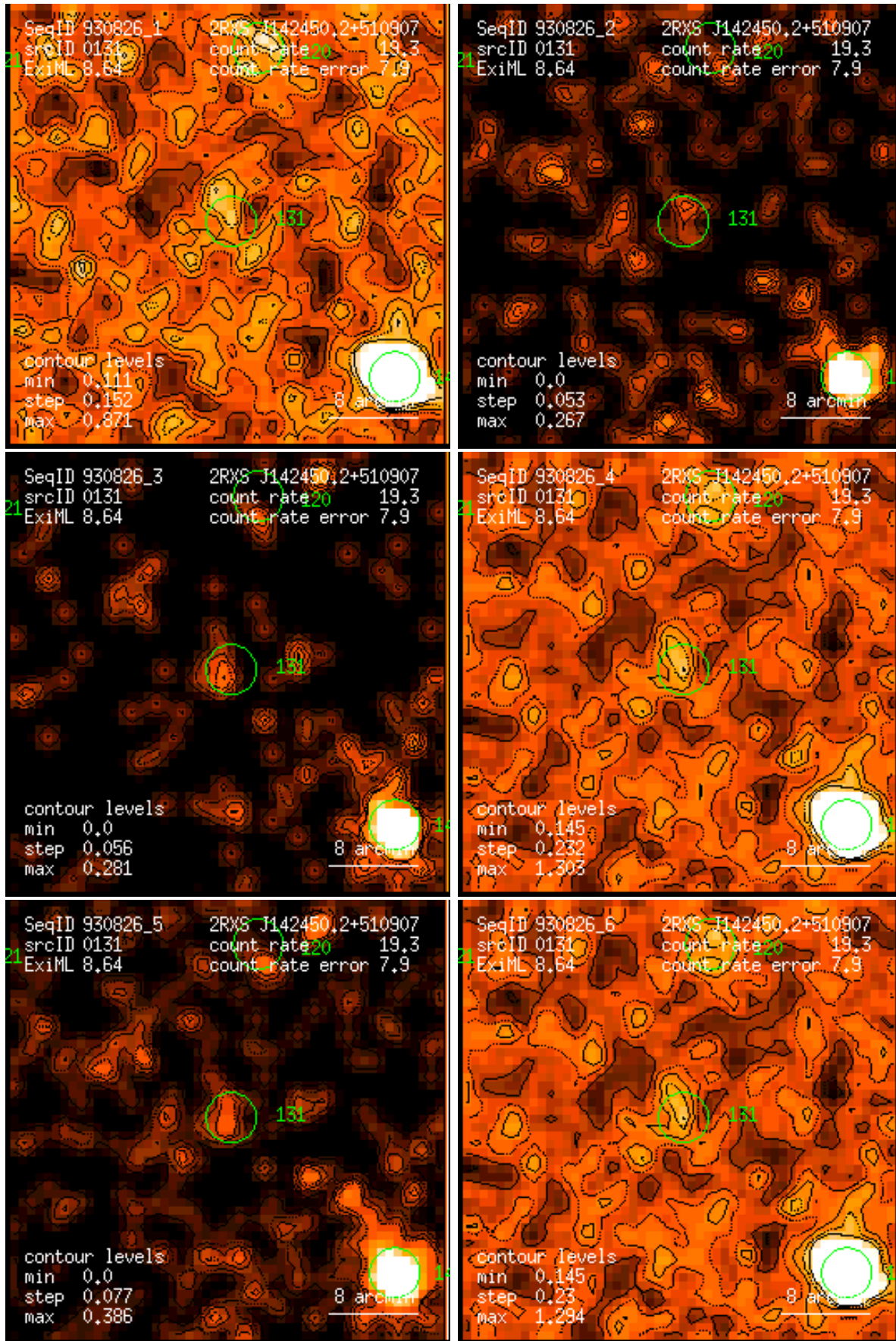
Figure 131: RASS 930826: detection 0131: band rate images, Gaussian filter: (1) PSPC channels 11 – 41, (2) 52 – 90, (3) 91 – 201, (4) 11 – 235, (5) 52 – 201, (6) 11 – 201. Broad band rates in counts/ks. Band rate contour levels in counts/ks/arcmin 2 .
