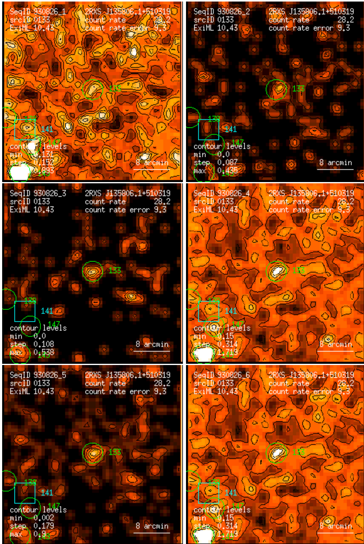
Figure 133: RASS 930826: detection 0133: band rate images, Gaussian filter: (1) PSPC channels 11 – 41, (2) 52 – 90, (3) 91 – 201, (4) 11 – 235, (5) 52 – 201, (6) 11 – 201. Broad band rates in counts/ks. Band rate contour levels in counts/ks/arcmin 2 .
