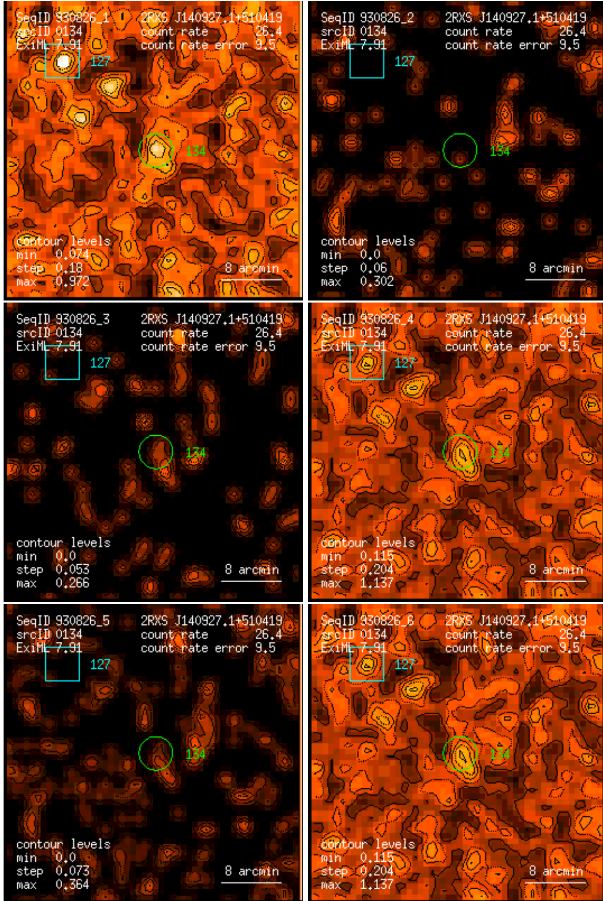
Figure 134: RASS 930826: detection 0134: band rate images, Gaussian filter: (1) PSPC channels 11 – 41, (2) 52 – 90, (3) 91 – 201, (4) 11 – 235, (5) 52 – 201, (6) 11 – 201. Broad band rates in counts/ks. Band rate contour levels in counts/ks/arcmin 2 .
