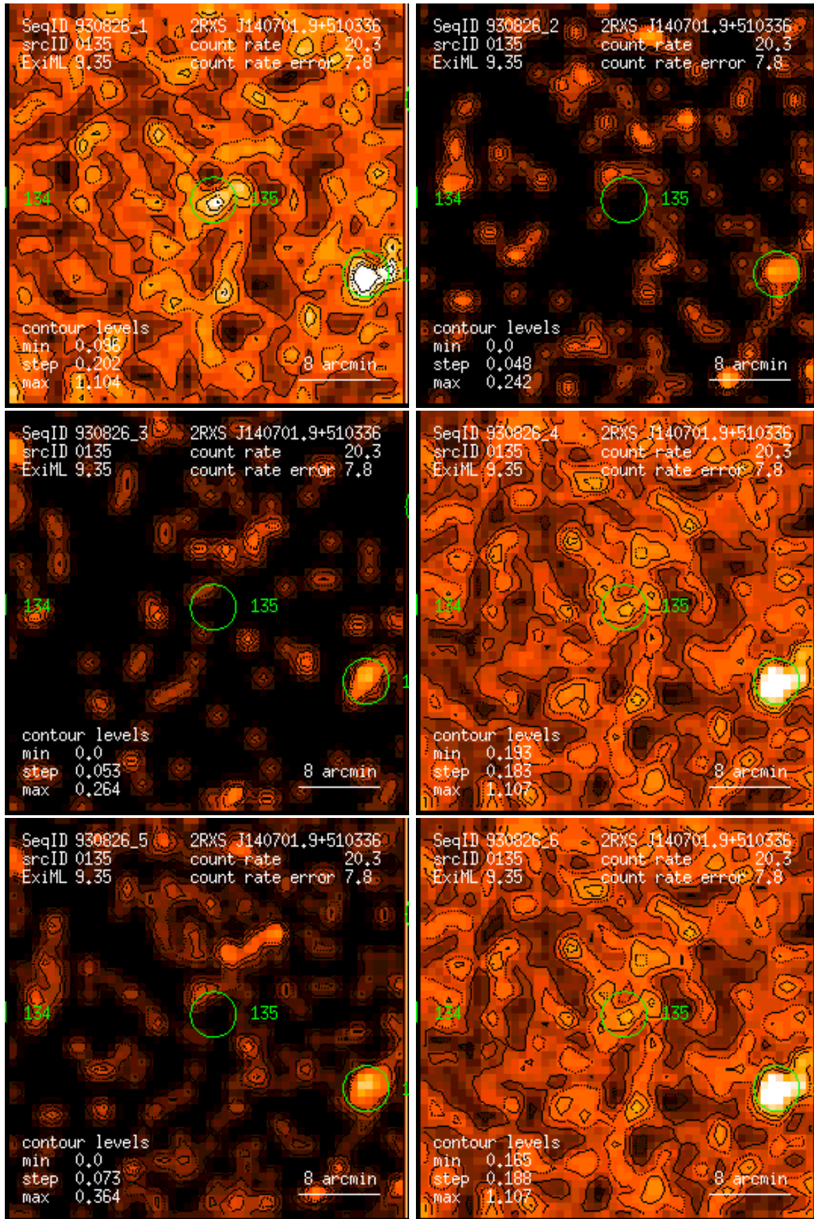
Figure 135: RASS 930826: detection 0135: band rate images, Gaussian filter: (1) PSPC channels 11 – 41, (2) 52 – 90, (3) 91 – 201, (4) 11 – 235, (5) 52 – 201, (6) 11 – 201. Broad band rates in counts/ks. Band rate contour levels in counts/ks/arcmin 2 .
