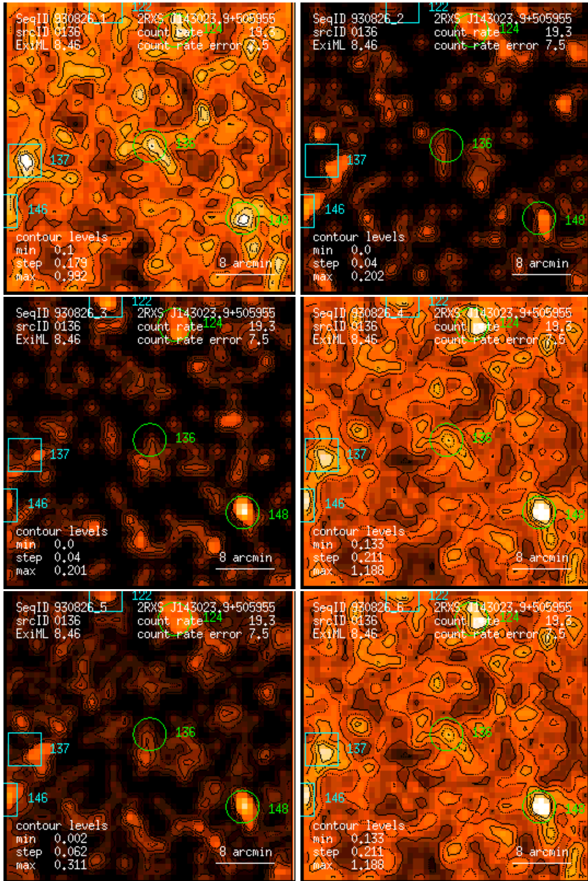
Figure 136: RASS 930826: detection 0136: band rate images, Gaussian filter: (1) PSPC channels 11 – 41, (2) 52 – 90, (3) 91 – 201, (4) 11 – 235, (5) 52 – 201, (6) 11 – 201. Broad band rates in counts/ks. Band rate contour levels in counts/ks/arcmin 2 .
