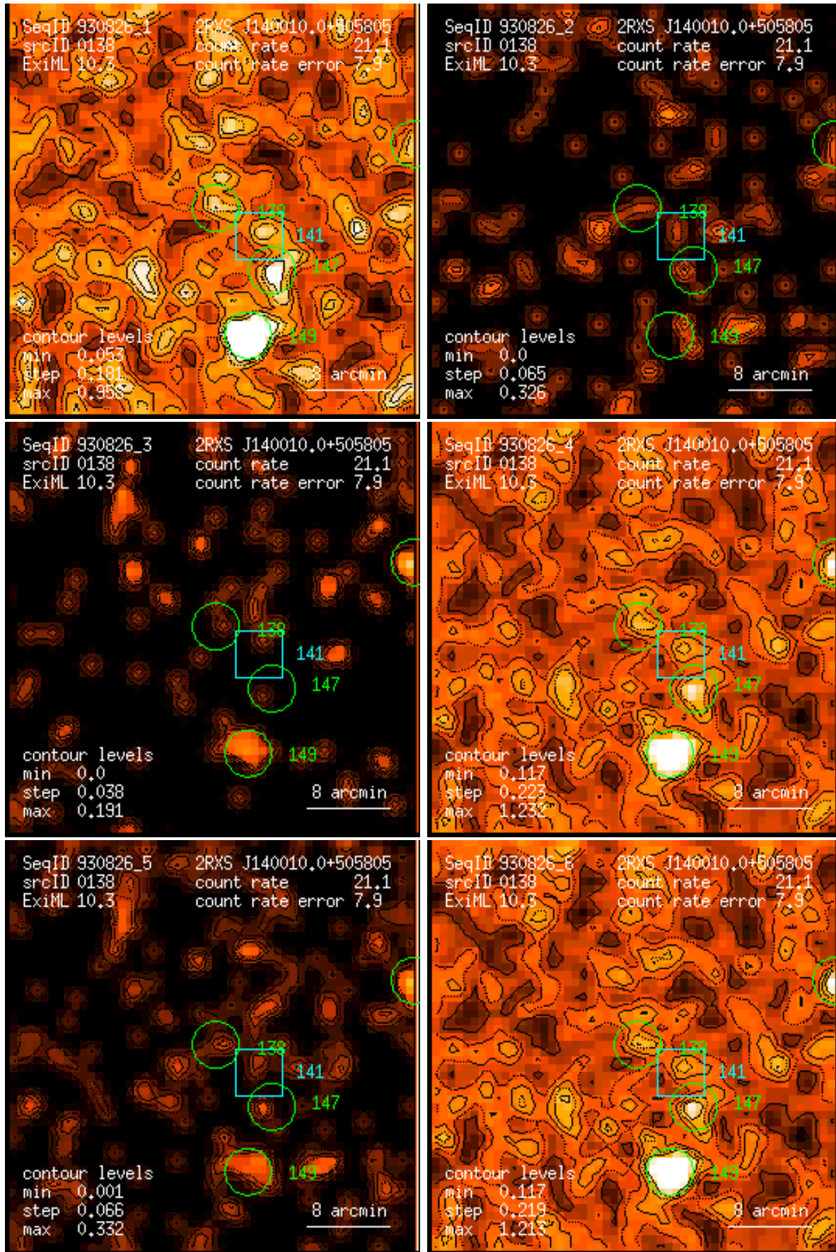
Figure 138: RASS 930826: detection 0138: band rate images, Gaussian filter: (1) PSPC channels 11 – 41, (2) 52 – 90, (3) 91 – 201, (4) 11 – 235, (5) 52 – 201, (6) 11 – 201. Broad band rates in counts/ks. Band rate contour levels in counts/ks/arcmin 2 .
