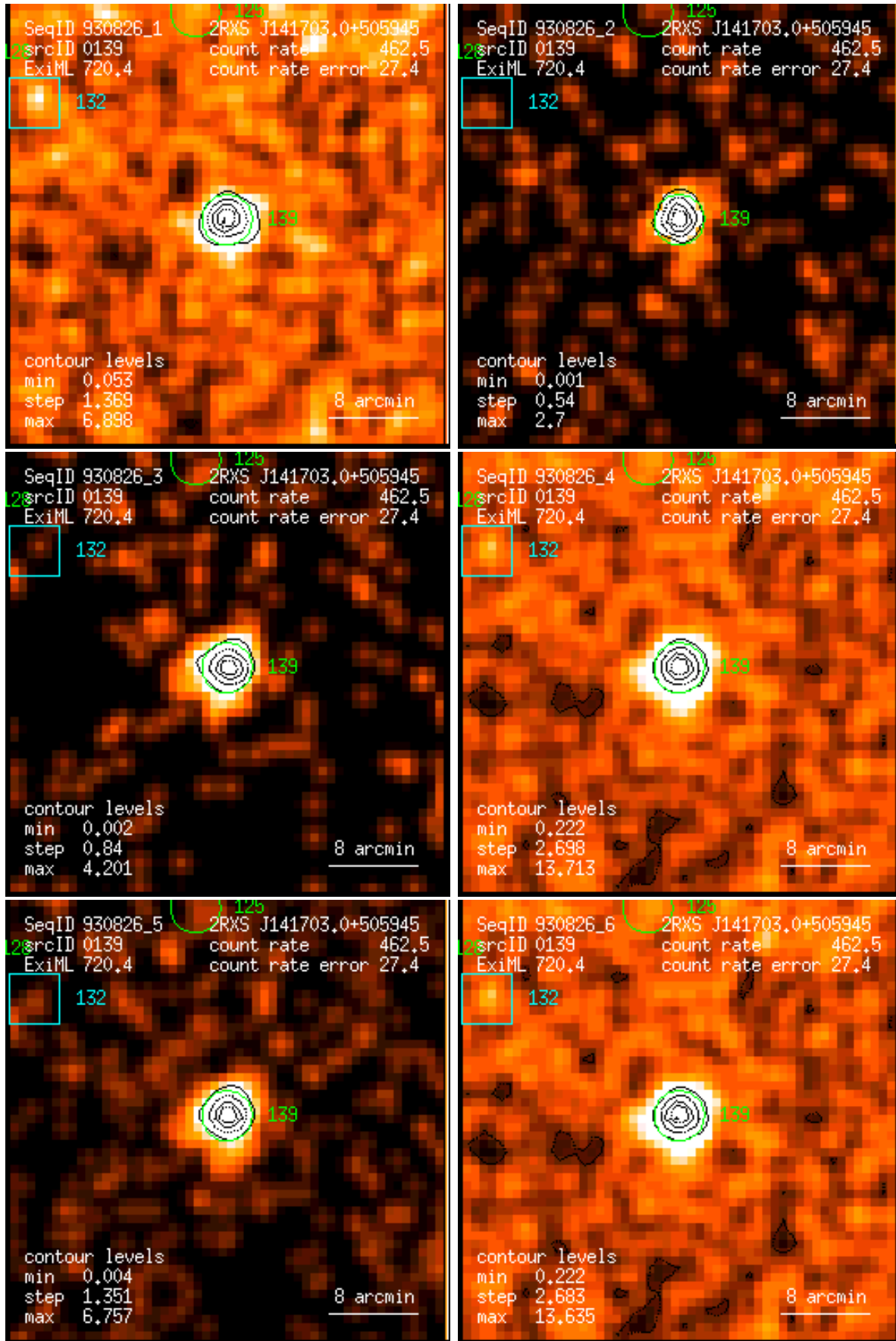
Figure 139: RASS 930826: detection 0139: band rate images, Gaussian filter: (1) PSPC channels 11 – 41, (2) 52 – 90, (3) 91 – 201, (4) 11 – 235, (5) 52 – 201, (6) 11 – 201. Broad band rates in counts/ks. Band rate contour levels in counts/ks/arcmin 2 .
