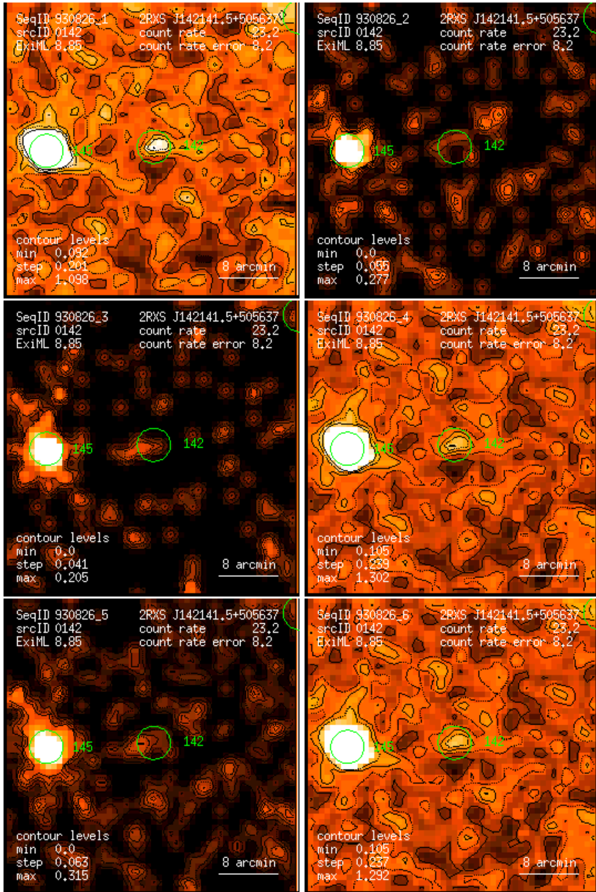
Figure 142: RASS 930826: detection 0142: band rate images, Gaussian filter: (1) PSPC channels 11 – 41, (2) 52 – 90, (3) 91 – 201, (4) 11 – 235, (5) 52 – 201, (6) 11 – 201. Broad band rates in counts/ks. Band rate contour levels in counts/ks/arcmin 2 .
