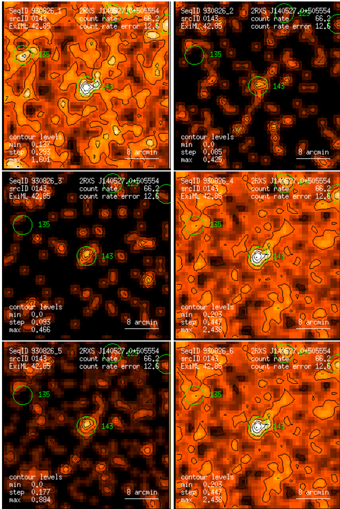
Figure 143: RASS 930826: detection 0143: band rate images, Gaussian filter: (1) PSPC channels 11 – 41, (2) 52 – 90, (3) 91 – 201, (4) 11 – 235, (5) 52 – 201, (6) 11 – 201. Broad band rates in counts/ks. Band rate contour levels in counts/ks/arcmin 2 .
