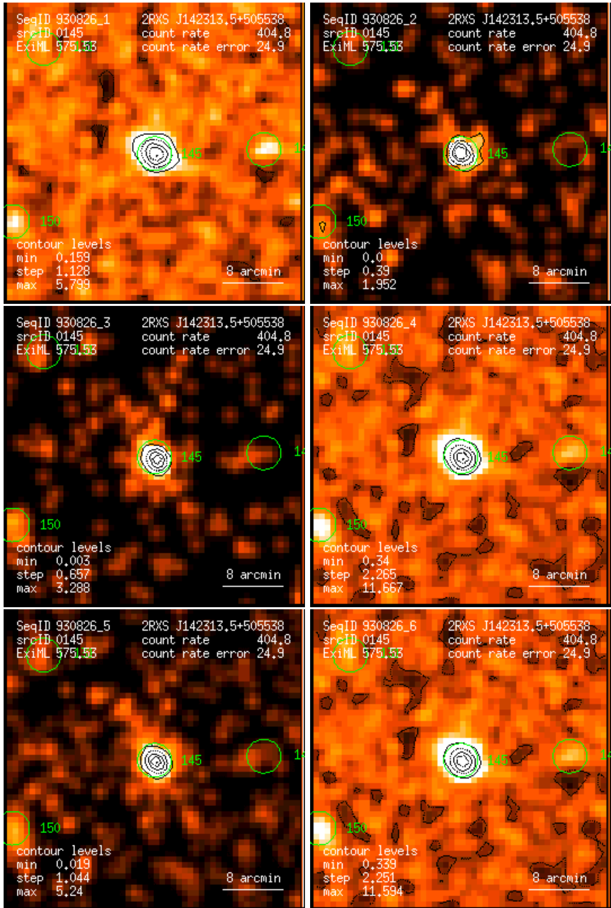
Figure 145: RASS 930826: detection 0145: band rate images, Gaussian filter: (1) PSPC channels 11 – 41, (2) 52 – 90, (3) 91 – 201, (4) 11 – 235, (5) 52 – 201, (6) 11 – 201. Broad band rates in counts/ks. Band rate contour levels in counts/ks/arcmin 2 .
