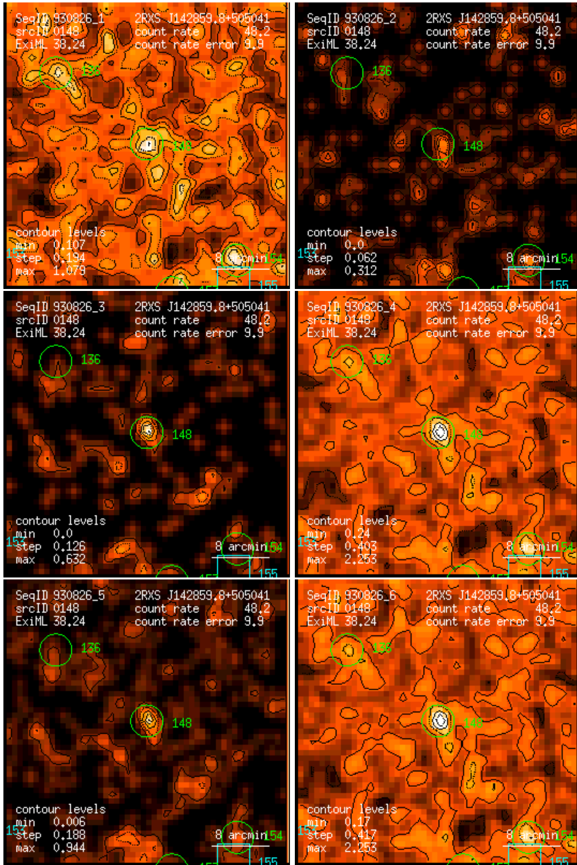
Figure 148: RASS 930826: detection 0148: band rate images, Gaussian filter: (1) PSPC channels 11 – 41, (2) 52 – 90, (3) 91 – 201, (4) 11 – 235, (5) 52 – 201, (6) 11 – 201. Broad band rates in counts/ks. Band rate contour levels in counts/ks/arcmin 2 .
