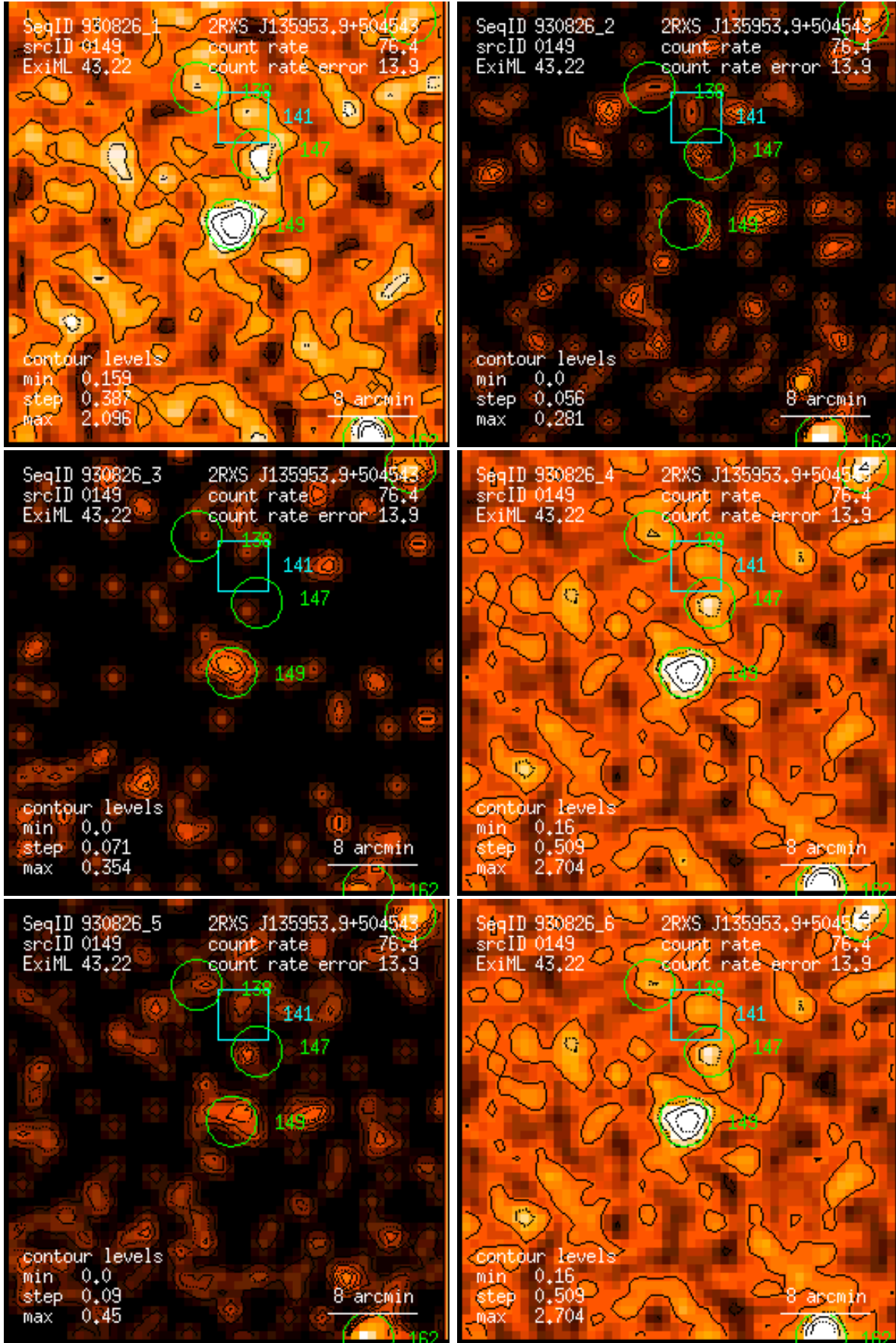
Figure 149: RASS 930826: detection 0149: band rate images, Gaussian filter: (1) PSPC channels 11 – 41, (2) 52 – 90, (3) 91 – 201, (4) 11 – 235, (5) 52 – 201, (6) 11 – 201. Broad band rates in counts/ks. Band rate contour levels in counts/ks/arcmin 2 .
