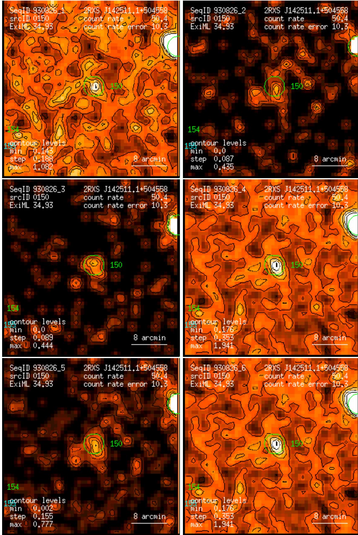
Figure 150: RASS 930826: detection 0150: band rate images, Gaussian filter: (1) PSPC channels 11 – 41, (2) 52 – 90, (3) 91 – 201, (4) 11 – 235, (5) 52 – 201, (6) 11 – 201. Broad band rates in counts/ks. Band rate contour levels in counts/ks/arcmin 2 .
