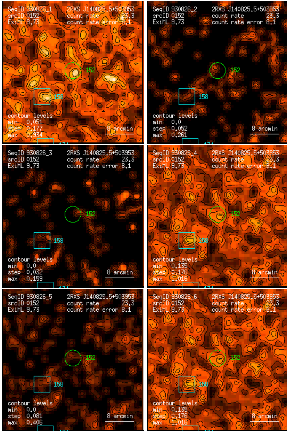
Figure 152: RASS 930826: detection 0152: band rate images, Gaussian filter: (1) PSPC channels 11 – 41, (2) 52 – 90, (3) 91 – 201, (4) 11 – 235, (5) 52 – 201, (6) 11 – 201. Broad band rates in counts/ks. Band rate contour levels in counts/ks/arcmin 2 .
