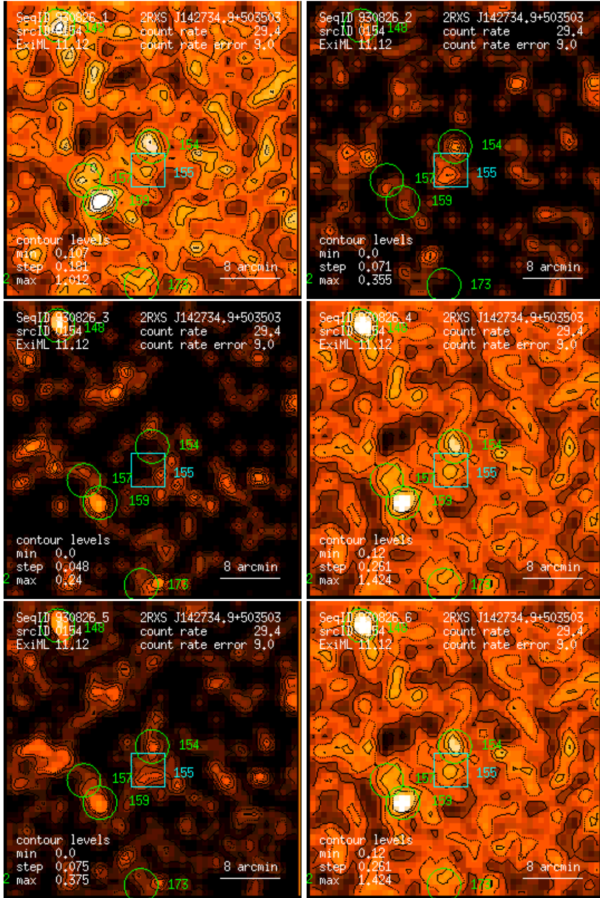
Figure 154: RASS 930826: detection 0154: band rate images, Gaussian filter: (1) PSPC channels 11 – 41, (2) 52 – 90, (3) 91 – 201, (4) 11 – 235, (5) 52 – 201, (6) 11 – 201. Broad band rates in counts/ks. Band rate contour levels in counts/ks/arcmin 2 .
