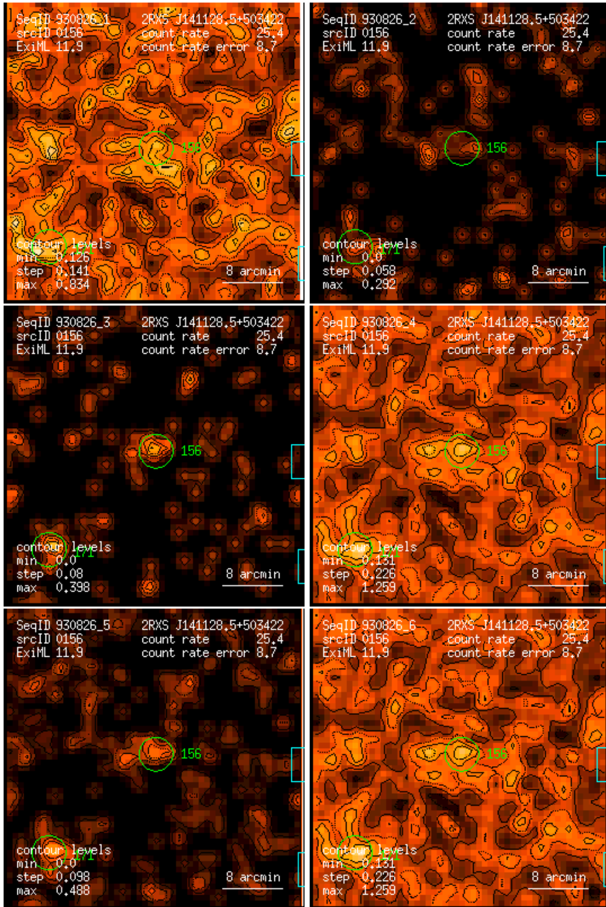
Figure 156: RASS 930826: detection 0156: band rate images, Gaussian filter: (1) PSPC channels 11 – 41, (2) 52 – 90, (3) 91 – 201, (4) 11 – 235, (5) 52 – 201, (6) 11 – 201. Broad band rates in counts/ks. Band rate contour levels in counts/ks/arcmin 2 .
